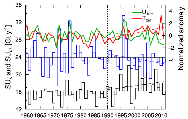
Fig. 10. Interannual variability (1960–2011) of GrIS integrated SU ds (blue bars) and SU s (black bars), combined with the normalized anomaly of GRIS averaged 10 m wind speed ( U_{10m} , green) and 2 m temperature ( T_{2m} , red). The 1990–2011 linear trends are depicted by the dashed lines.
