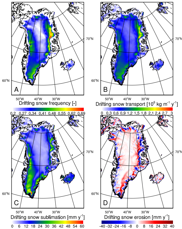
Fig. 5. Mean drifting snow frequency (A), transport (B), sublimation (C) and erosion (D). Drifting snow frequency is defined as the fraction of days with accumulated TR_{ds} of 3 \text{ kg m}^{-1} . Dashed-dotted lines represent the topography with 500 m intervals.
