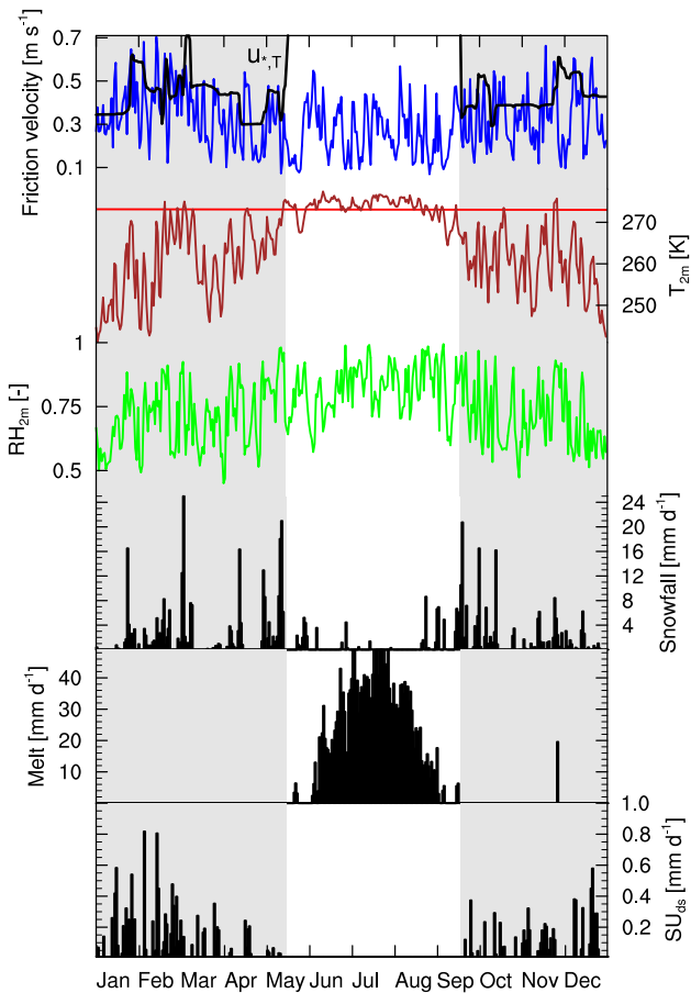
Fig. 9. Modeled annual cycle (2005) at S6 (67°5' N, 49° 23' W) of daily mean friction velocity (blue) and its threshold (black, see text), 2 m temperature (the freezing point is illustrated by the horizontal red line) and relative humidity, daily accumulated snowfall, snowmelt and drifting snow sublimation. The grey areas represent the drifting snow season (see text).
