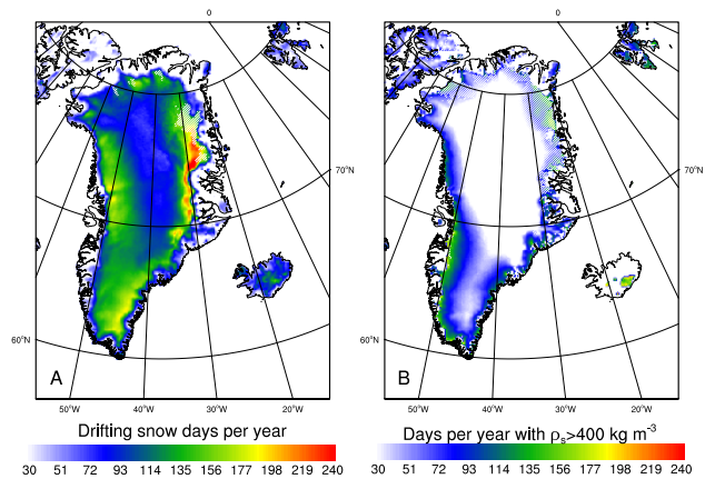
Fig. 8. Number of drifting snow days (with SU_{ds} > 0 ) per year and number of days with snow density of the upper 5 cm of the snowpack ( \rho_s > 400\ kg\ m^{-3} ). White dashes indicate areas with a standard deviation > 30 days.
