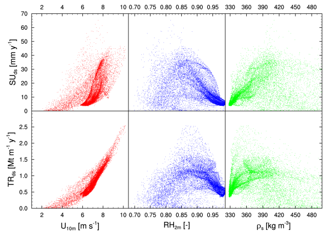
Fig. 6. Mean (1960–2011) SU_{ds} and TR_{ds} on all ice sheet grid points ( \sim 14\,000 points) as a function of mean 10 m wind speed (red), 2 m relative humidity with respect to ice (blue) and surface snow density (green).
