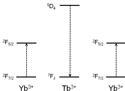
Fig. 4. Cooperative energy transfer from Tb to two Yb ions. From the ^5\text{D}_4 state of one Tb ion two neighbouring Yb ions are excited to the 2\text{F}_{5/2} state from where emission of 980 \text{ nm} photons can occur (after Meijerink et al. 2006, Vergeer et al. 2005).
