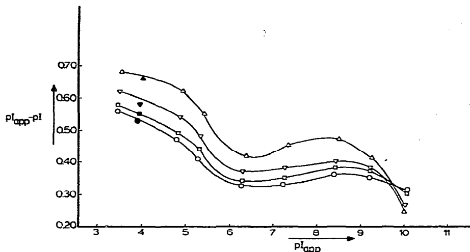
Fig. 1. Values of pI_{app} - pI versus pI_{app} for Amphotolines (open symbols) and Servaltes (closed symbols) at 25° in 6 M solutions of urea in water (○) and sucrose-water mixtures containing 15 (□), 30 (▽) and 45% (w/w) (△) sucrose.
