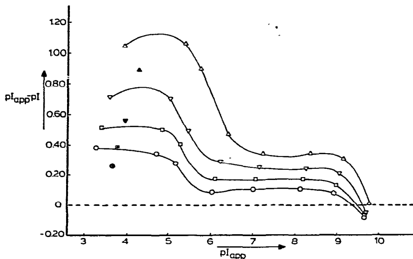
Fig. 2. Values of pI_{app} - pI versus pI_{app} for Amphotolines (open symbols) and Servaltes (closed symbols) at 25° in 30% (w/w) solutions of ethanol in water (○) and glycerol-water mixtures containing 20 (□), 40 (▽) and 60% (w/w) (△) glycerol.
