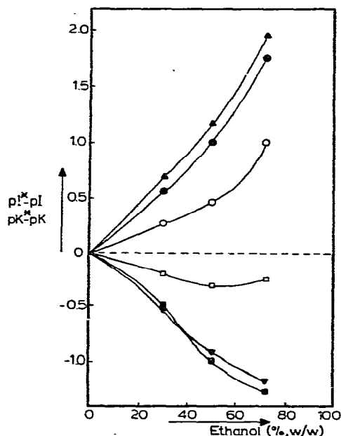
Fig. 5. Values at 25° of pK^* - pK for acetic acid (●), propionic acid (▲), n -butylammonium ion (■) and n -propylammonium ion (▼) and pI^* - pI for Amphotines, pI = 2.90 (○) and pI = 9.76 (□), in ethanol-water mixtures.
