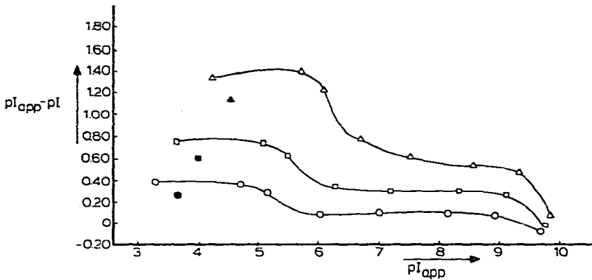
Fig. 4. Values of pI_{app} - pI versus pI_{app} for Ampholines (open symbols) and Servalyte (closed symbols) at 25° in aqueous solutions containing 30 (○), 50 (□) and 72% (△) ethanol.
