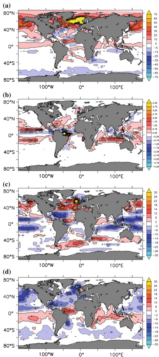
Fig. 4 As in Fig. 2, but for the large-scale regression parameter p_2 . The units are the same of Fig. 2, divided by °C In panel a, only the non-solar heat flux is considered. In panel b, the signal of the freshwater pulse has been removed from the source data
