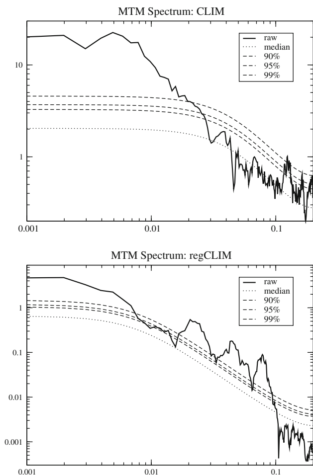
Fig. 10 MTM spectra of the time series of the maximum AMOC (solid lines) for CLIM (top panel) and regCLIM (bottom panel). The dashed smooth lines represent, from the lowest to the highest, the estimated red noise background and the median, 90, 95 and 99% significance levels associated with it. In both cases, the resolution is (5 \text{ years})^{-1} and 7 tapers were used. Time series are 1,000 years long
