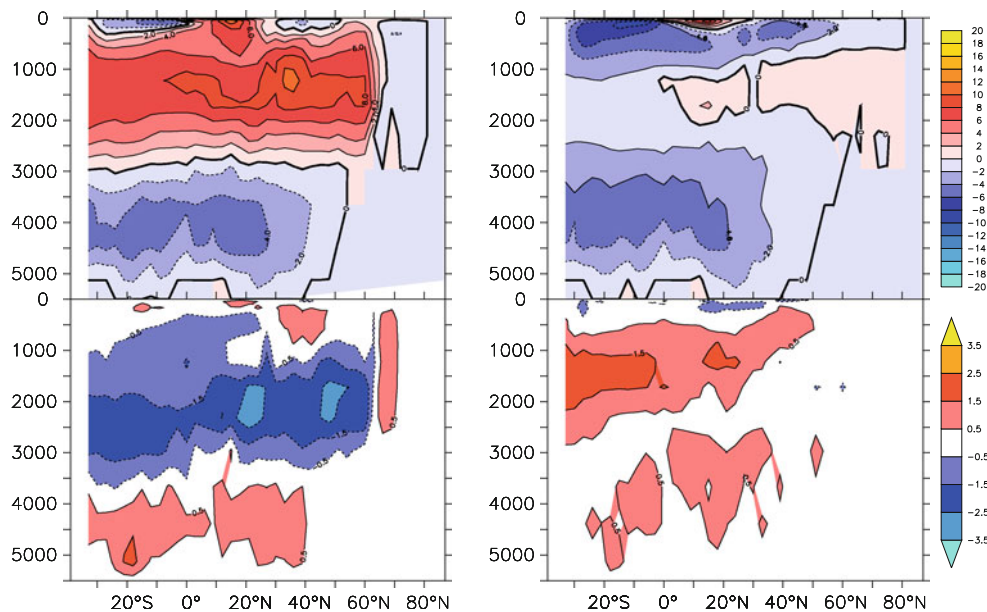
Fig. 8 Overview of overturning streamfunction in the various models. In the top panels , AMOC for the CLIM mean state ( top left ) and for years 101 to 110 of PULSE ( top right ) are shown. The shaded contours are every 2 Sv, the red filling is for positive values, blue for negative. The thick line is the zero contour. In the left bottom
