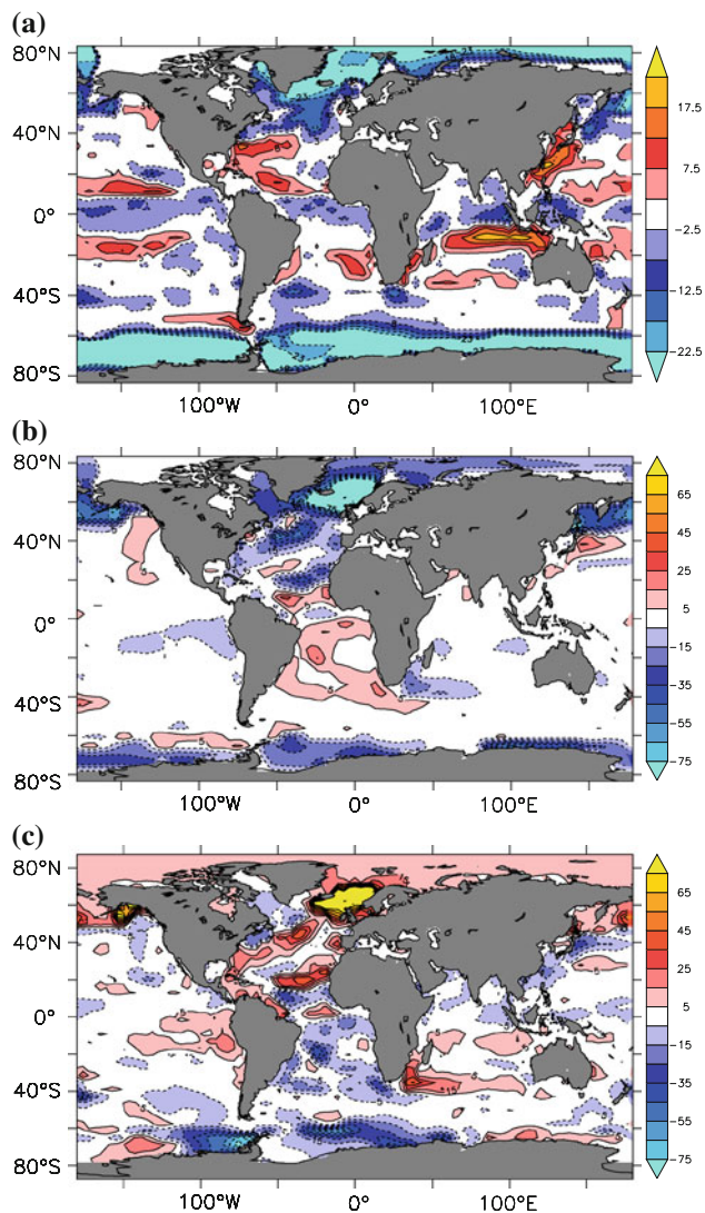
Fig. 6 Effective feedbacks for heat flux (short wave radiation excluded), when changes in sea-ice are considered (see text). Effective regression parameters for the heat flux, computed including the effect of changes in sea-ice ( p_1 in panel a and p_2 in panel b). Also the change in the heat flux, as directly diagnosed from the coupled model, is shown in panel c, computed as the difference in ice-weighted heat flux from years 91–100 and 1–10 of PULSE. Note that a different color scale is used in the top panel
