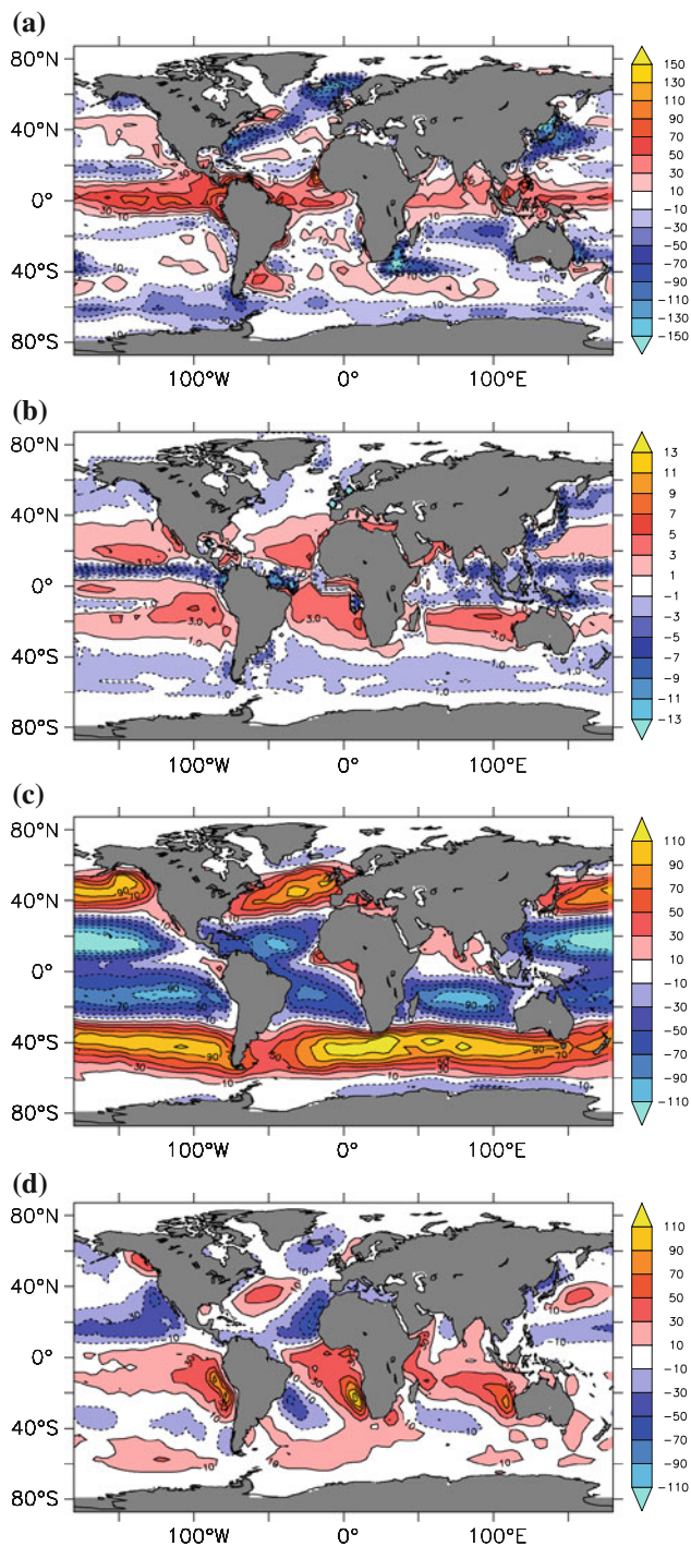
Fig. 2 Average value of the regressed fields from CLIM data ( \overline{\phi(i,j)} in Eq. 5), weighted by the fractional ocean area ( 1 - \varepsilon(i,j) ). a Total heat flux in \text{W/m}^2 , positive downwards. b Net evaporation in \text{mm/day} . c and d are the zonal and meridional components of wind-stress respectively, in 10^{-3} \times \text{N/m}^2
