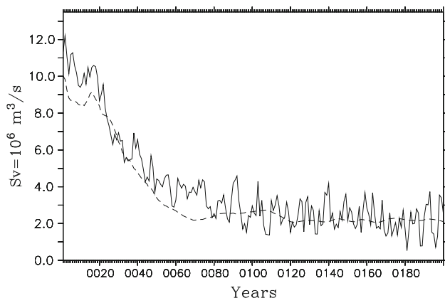
Fig. 11 Maximum AMOC for first 200 years of PULSE (full line) and regPULSE (dashed line) in Sv
