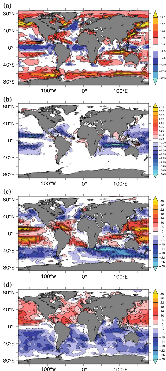
Fig. 3 As in Fig. 2, but for the local regression parameter p_1 . The units are the same of Fig. 2, divided by ^\circ\text{C} . In panel a , only the non-solar heat flux is considered
