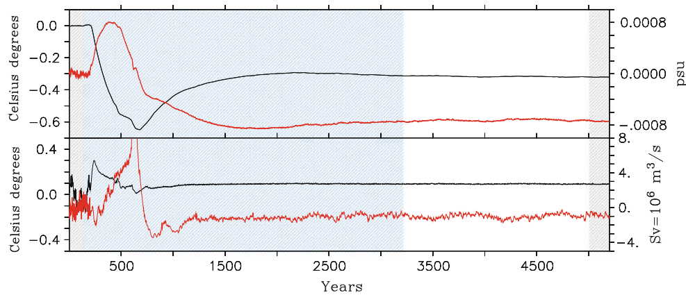
Fig. 7 Deviation from CLIM average in regCLIM of four quantities: global average sea temperature ( top panel, black, left y-axis ), global average salinity ( top panel, red, right y-axis ), global average SST ( bottom panel, black, left y-axis ) and maximum AMOC ( lower panel, red, right y-axis )
