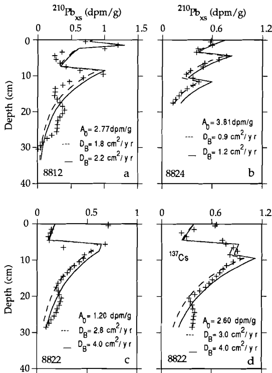
Fig. 8 The distribution of ^{210}\text{Pb} in cores 8812 and 8824, and the ^{210}\text{Pb} and ^{137}\text{Cs} in core 8822. Solid and dashed lines are calculated best-fit curves for the subsurface egestion model. See text for discussion.
