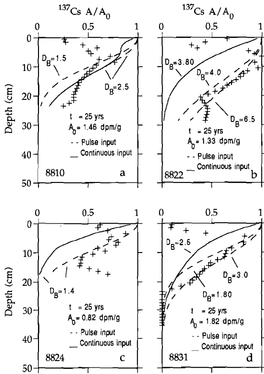
Fig. 7 ^{137}\text{Cs} activity-depth profiles (normalized to the A_0 ) in cores 8810, 8822, 8824 and 8831. Lines show model generated curves for the pulse input (dashed line) and the continuous input (solid line) models. Crosses are measured data. See text for discussion.
