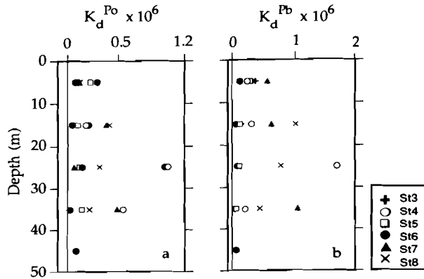
Fig. 7 The vertical profiles of (a) ^{210}\text{Po} distribution coefficient, (b) ^{210}\text{Pb} distribution coefficient.
