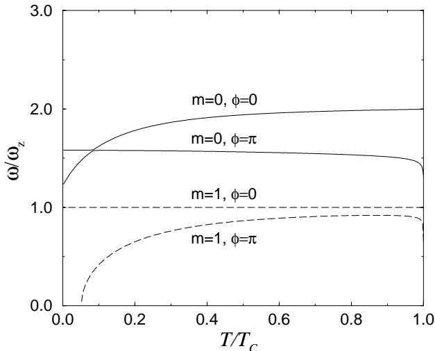
FIG. 3. The in-phase and out-of-phase m = 0 (solid lines), and Kohn (dashed lines) modes as a function of T/T_c for the experimental conditions of Stamper-Kurn et al. [9], with a total number of particles N = 40 \times 10^6
