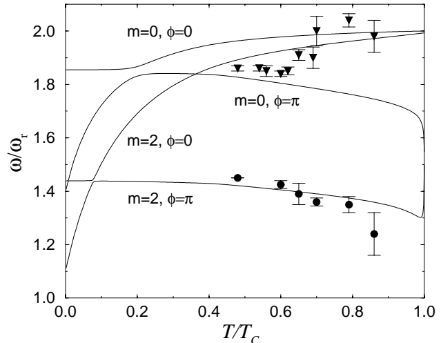
FIG. 1. The in-phase and out-of-phase m = 0, 2 modes as a function of T/T_c for the experimental conditions of Jin et al. [10]. The relative phase of the density profiles of the condensed and noncondensed atoms is denoted by \phi . Also included are the experimental results for the m = 0 (triangles) and m = 2 (circles) modes found in these experiments.
