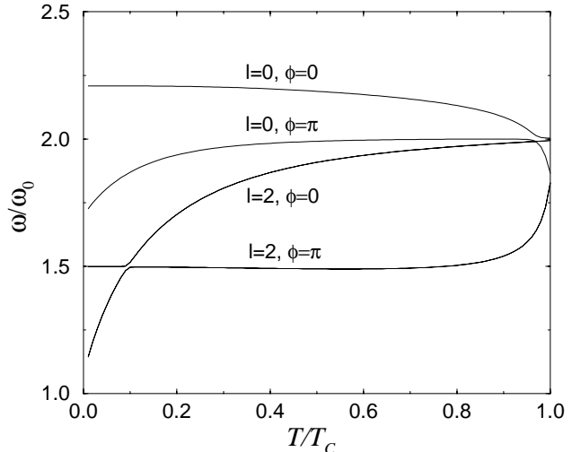
FIG. 4. The in-phase and out-of-phase m = 0, 2 modes as a function of T/T_c for an isotropic trap \omega_x = \omega_y = \omega_z = \omega_0 = 200\text{Hz} and with a total number of atoms N = 2000 .
