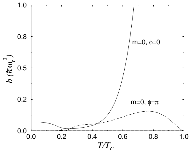
FIG. 2. The residue b for the modes m = 0, \phi = 0 (solid line) and m = 0, \phi = \pi (dotted line) as a function of T/T_c for the experimental conditions of Jin et al. [10].
