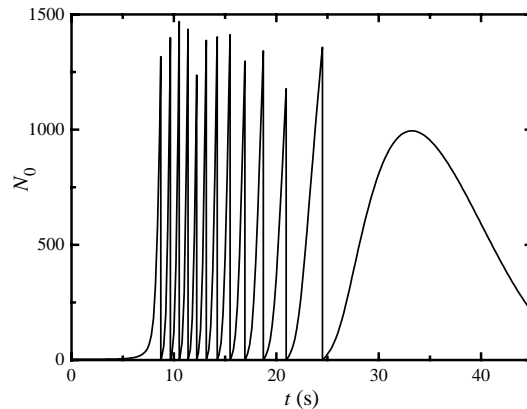
FIG. 3. Typical evolution of condensate number N_0 in response to evaporative cooling. The gas initially consists of 4 \times 10^5 atoms at 500 nK. During the first 5 seconds of evolution, roughly 40% of the atoms are removed by evaporative cooling, after which evaporation is halted.
