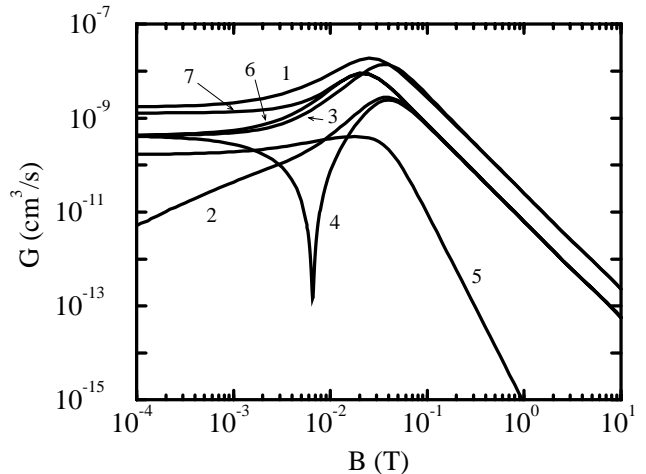
FIG. 2. Exchange decay rate constants for the processes 1) 65 \rightarrow 61 , 2) 54 \rightarrow 63 , 3) 54 \rightarrow 52 , 4) 54 \rightarrow 41 , 5) 54 \rightarrow 21 , 6) 64 \rightarrow 62 , 7) 64 \rightarrow 51 as a function of the magnetic field strength.
