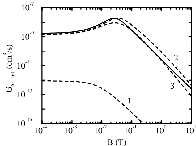
FIG. 4. Exchange decay rate G_{65 \rightarrow 61} of the {}^6\text{Li} gas. The solid line gives the CC result. The dashed lines represent 1) the DIS approximation, 2) the ABC approximation with R = 40a_0 , and 3) the ABC approximation with R = 60a_0 .
