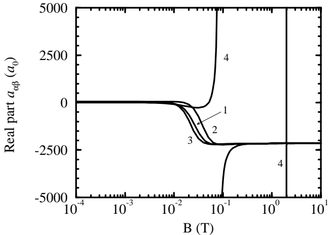
FIG. 1. Real part of zero-temperature s -wave scattering length for 1) 65, 2) 54, 3) 64, and 4) 21 collisions as a function of the magnetic field.
