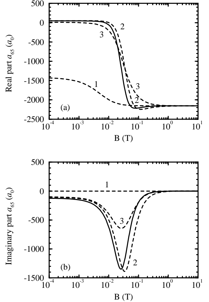
FIG. 3. The a) real and b) imaginary part of the s -wave scattering length a_{65} . The solid line is the CC value, which goes to the triplet scattering length for large magnetic fields. The dashed lines are 1) the DIS approximation, 2) the ABC approximation with R = 40a_0 , and 3) the ABC approximation with R = 60a_0 .
