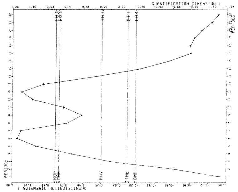
Figure 6: analysis 2, category and period quantifications, 22 x 5 table
