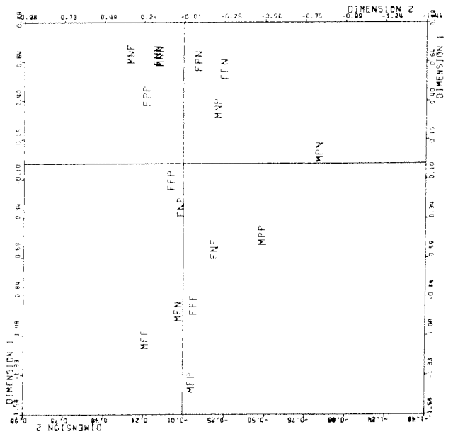
Figure 3: analysis 1, centroids for passive sex x work variable
