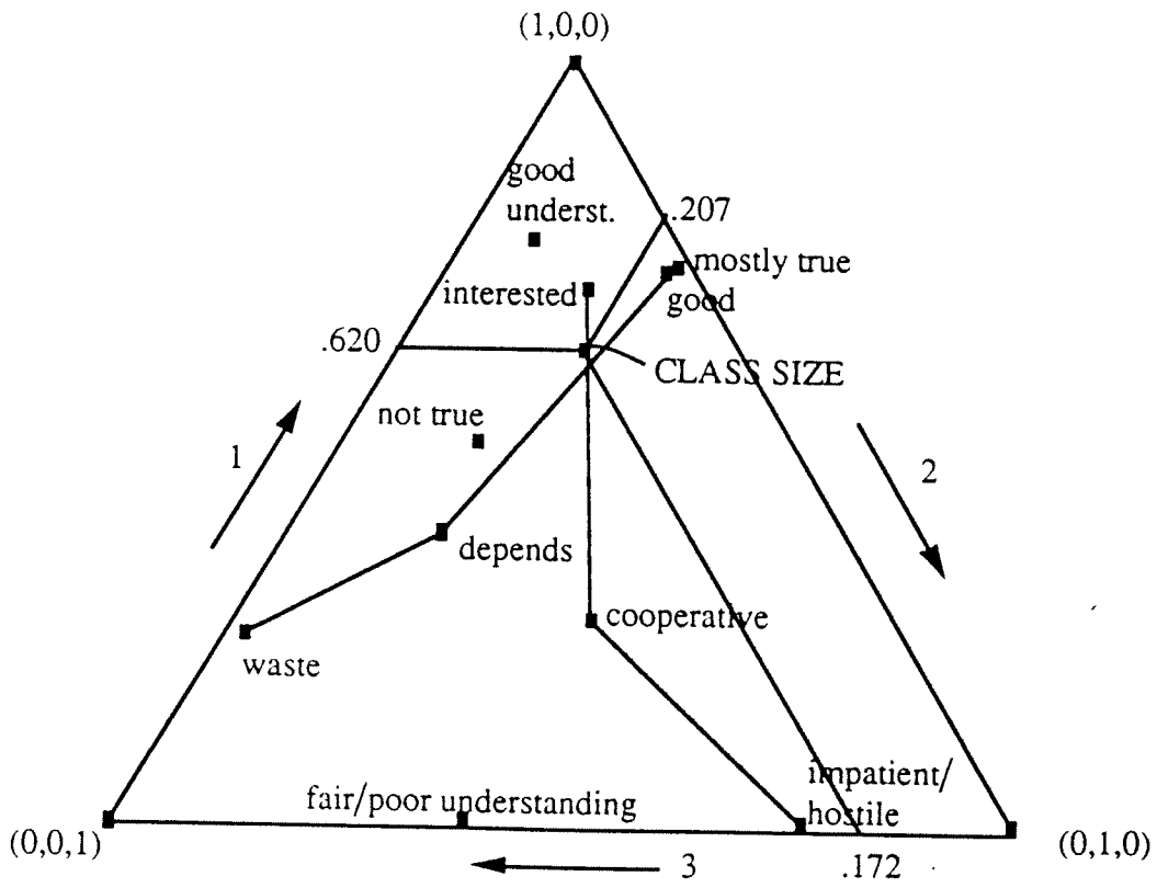
Figure 4: Latent class analysis, rescaled parameter estimates
