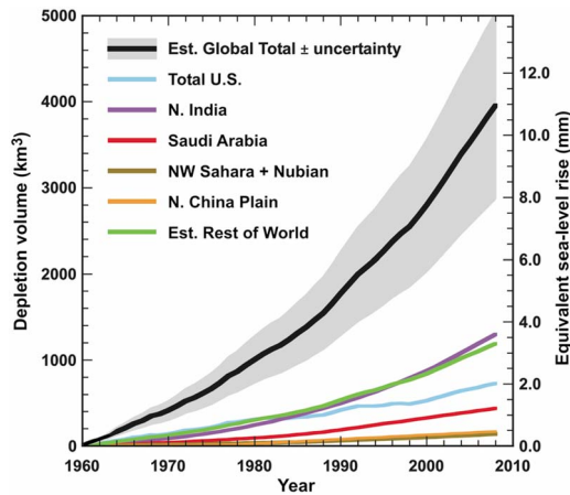
Figure 1. Cumulative net groundwater depletion, 1961–2008.
