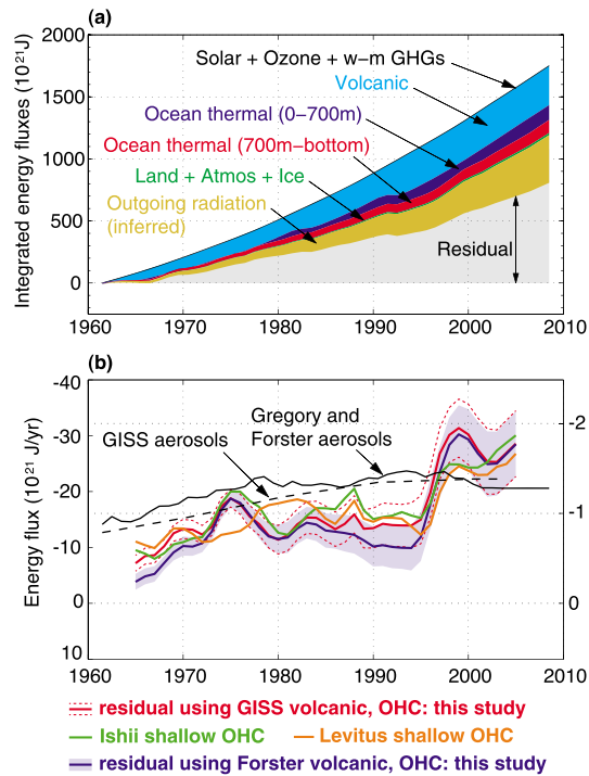
Figure 3. The Earth's energy budget from 1961 through 2008. (a) The top line indicates the integrated radiative forcing from well-mixed greenhouse gases, ozone and solar changes. This radiative forcing is offset by the cooling due to stratospheric aerosols from volcanic eruptions (cyan), the warming of the upper (0 to 700 m) ocean (blue), the deep ocean (red) and energy absorbed in the melting of ice and warming the atmosphere and the land (green), and the change in outgoing radiation inferred from temperature change (brown). The integrated aerosol (and other) forcing is estimated as a residual (grey). (b) The inferred global averaged aerosol radiative cooling (red) is calculated for three different values of \lambda [ 1.25 \text{ W m}^{-2} \text{ K}^{-1} (solid) and 0.75 \text{ W m}^{-2} \text{ K}^{-1} and 1.75 \text{ W m}^{-2} \text{ K}^{-1} (dashed)]. The aerosol coolings for the central value of \lambda are also given for the Ishii and Kimoto [2009] and Levitus et al. [2009] heat content estimates (green and orange respectively). The equivalent results for the Gregory and Forster [2008] volcanic forcing and the present heat content estimates are shown by the blue line and shading. Results from previous aerosol forcing estimates of Gregory and Forster [2008] and GISS forcing are shown in black solid and dashed respectively.
