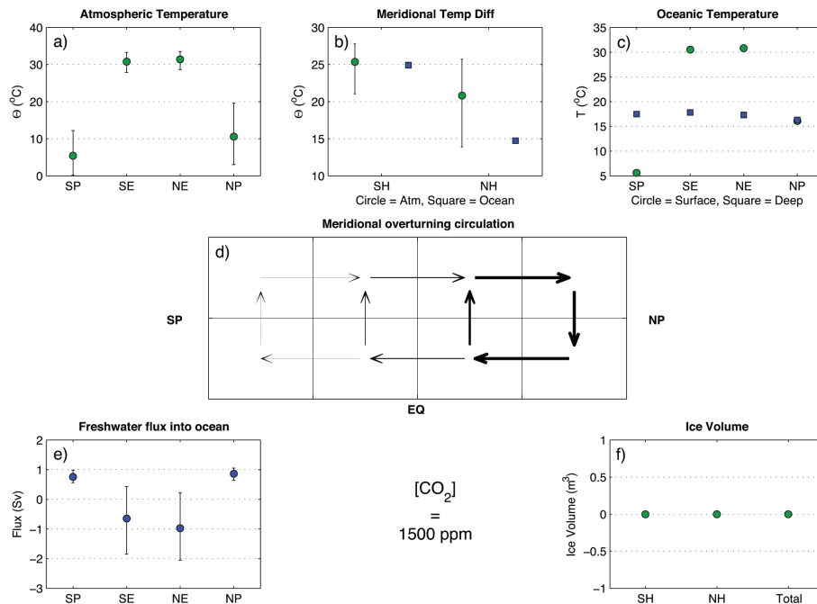
Fig. 5. Overview of the modelled state of the Eocene climate at a CO 2 concentration of 1500 ppm with the MOC in the NPP pattern; (a) atmospheric temperature for the southern polar (SP), southern equatorial (SE), northern equatorial (NE) and northern polar (NP) boxes; (b) meridional temperature difference for the Southern Hemisphere (SH) and Northern Hemisphere (NH) for the atmosphere (circles) and ocean (squares); (c) oceanic temperature of surface waters (circles) and deep sea (squares); (d) northern sinking MOC where the direction of the arrows indicates the direction of volume transport and their thickness indicates the magnitude; (e) freshwater flux into the ocean; (f) ice volume on the Southern Hemisphere (SH), Northern Hemisphere (NH) and in total; markers represent yearly averaged values, error bars indicate the seasonality.
