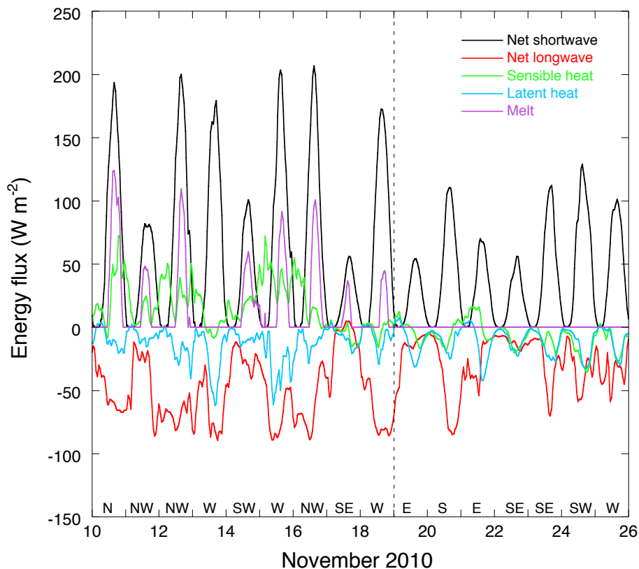
Fig. 12. Selected SEB components between 10 and 26 November 2010. Daily-mean wind direction is shown at the bottom of the panel.
