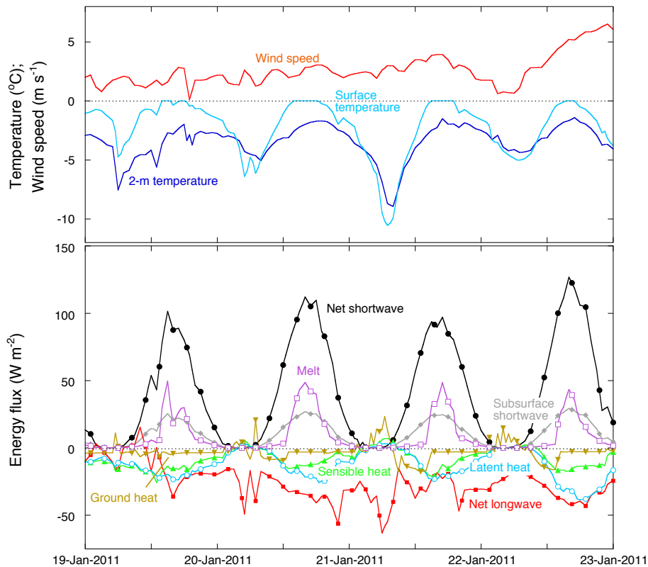
Fig. 9. Meteorological conditions (upper panel) and selected SEB components (lower panel) during a four-day period showing typical daytime convection.
