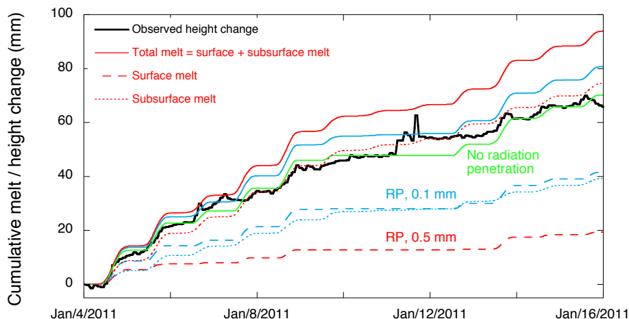
Fig. 8. Comparison of observed cumulative height change and modeled cumulative melt at AWS 14, for different model settings of radiation penetration. Observed height change (converted to mm w.e. assuming a density of 400 \text{ kg m}^{-3} ) shown in black; model without radiation penetration in green; model with radiation penetration (0.1 mm snow grain radius) in blue; model with radiation penetration (0.5 mm snow grain radius) in red. Dotted lines indicate subsurface melt; dashed lines indicate surface melt; and solid lines indicate total melt (= surface + subsurface melt).
