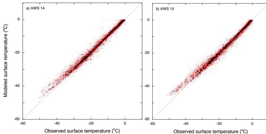
Fig. 5. Model performance check by comparing observed values of surface temperature to computed values, for (a) AWS 14; and (b) AWS 15. Red dots are hourly values, whereas black dots are daily-mean values.
