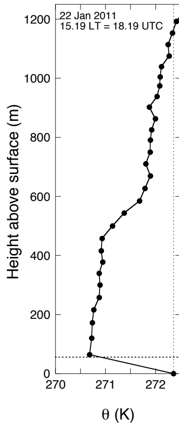
Fig. 10. Vertical profile of potential temperature (in K) from a radiosonde launched on 22 January 2011 at 15:19 LT (= 18:19 UTC). The horizontal dashed line indicates the height at which d\theta/dz changes sign, while the vertical dashed line illustrates that possible convection extends up to 1150 m, the height at which potential temperature equals surface potential temperature.
