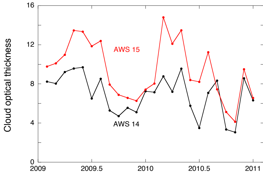
Fig. 4. Monthly means of cloud optical thickness (see text) at AWS 14 (black) and 15 (red).
