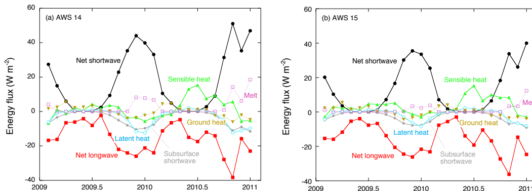
Fig. 6. Monthly means of surface energy budget components (in W m^{-2} ) for (a) AWS 14; and (b) AWS 15.
