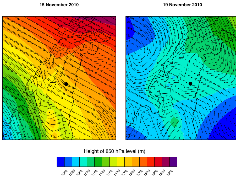
Fig. 11. Surface wind speed and direction (vectors) and the height of the 850 hPa level from RACMO2, for (a) 15 November 2010 and (b) 19 November 2010. The location of AWS 14 is denoted with the black dot.
