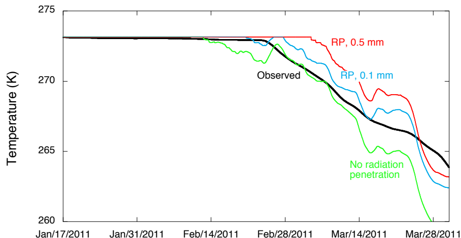
Fig. 7. Comparison between observed and modeled snow temperature at 0.5 m depth at AWS 14, for different model settings of radiation penetration. Observed snow temperature (interpolated to 0.5 m) shown in black; model without radiation penetration in green; model with radiation penetration (0.1 mm snow grain radius) in blue; model with radiation penetration (0.5 mm snow grain radius) in red.
