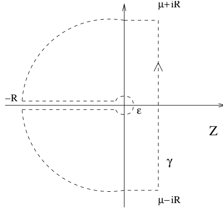
Figure 13: The Bromwich-Hankel contour used for the inverse Laplace transform. Integrating the function e^{ZA_1}/\sqrt{Z} along this contour, we obtain (A-32) in the limit R \rightarrow \infty, \epsilon \rightarrow 0 .
