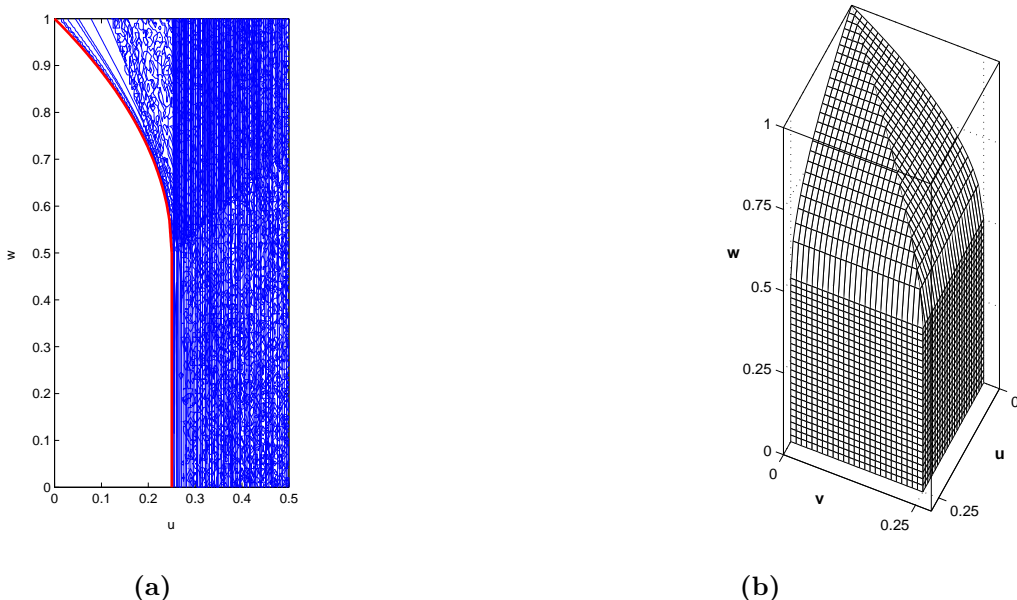
Figure 7: (a) : The critical line, combined from u = 1/4 , w = \lambda_+(u) , together with plots of the zeros of |P_{N,\{q\}}| for random sequences \{q\} and for sequences AB^{N-1} and A^{\frac{N}{2}}B^{\frac{N}{2}} at different values of N , in the u = v plane. (b) : The plot of the critical surface in the full parameter space of the (u, v, w) .
