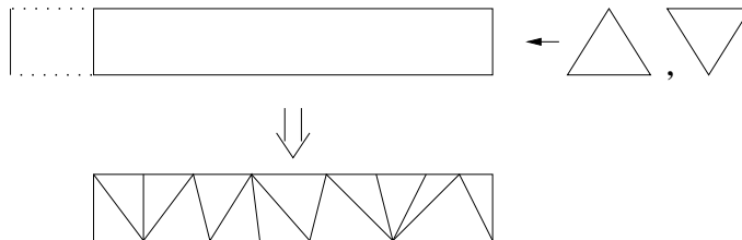
Figure 1: A triangulated strip constructed as a tower over a one-dimensional link.
