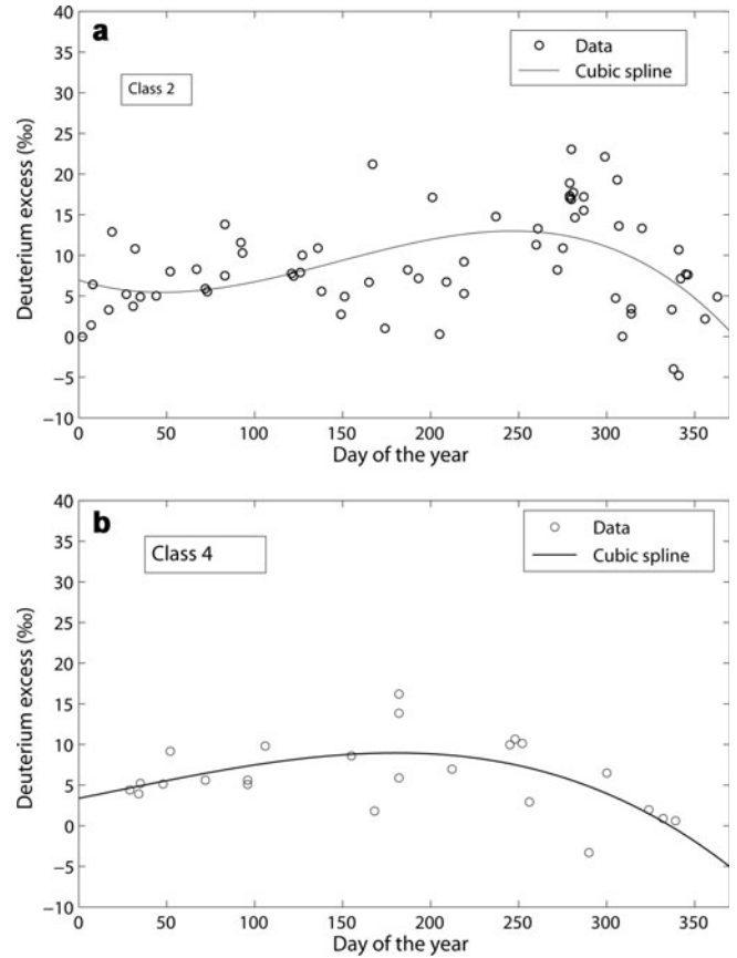
Fig. 4. Annual cycle of deuterium excess of surface snow samples at Neumayer station in the period 1981–2000: (a) for trajectory class 2, (b) for trajectory class 4. For easier comparison with the model results, the data are shown together with cubic splines through the data points (see explanation in the text).
