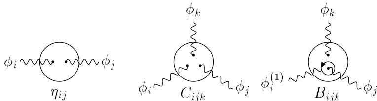
FIGURE 1: Closed string interactions.
