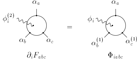
FIGURE 4: Deformation of the product.
