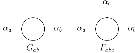
FIGURE 2: Open string interactions.
