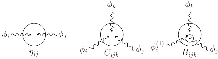
FIGURE 1: Closed string interactions.
