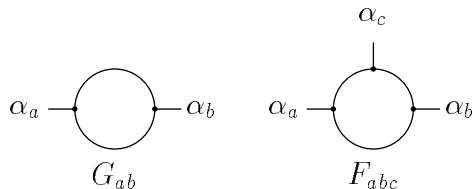
FIGURE 1: Closed string interactions.
