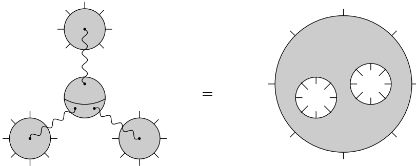
FIGURE 8: An open string loop diagram.
