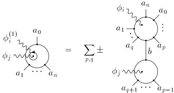
FIGURE 7: Factorisation of the bracket.
