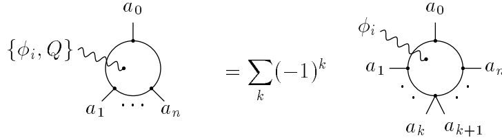
FIGURE 5: Factorisation of the BRST operator.
