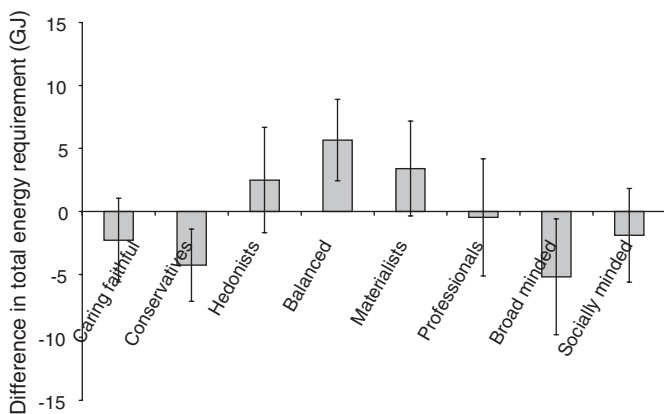
Fig. 3. The difference between total reference and total actual energy requirement ( \Delta E ) for the eight value groups, including the standard deviation of the mean.
