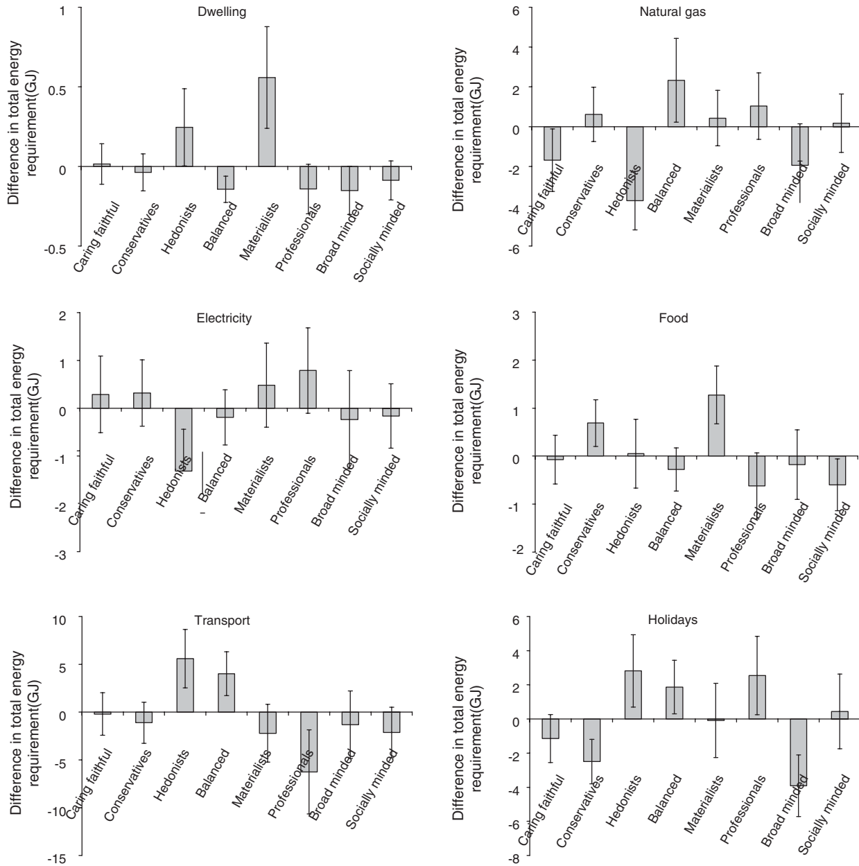
Fig. 4. For all six groups of consumption categories the difference between reference and actual energy requirement ( \Delta E ) for the eight value groups, including the standard deviation of the mean. Note that the vertical scales differ.
