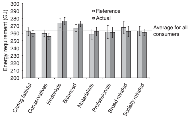
Fig. 2. The total reference energy requirement and total actual energy requirement for the eight value groups, including the standard deviation of the mean. The standard deviation from the mean is calculated by dividing the standard deviation by the square root of N (here N varies between 190 and 497 depending on the value group). This implies that the error intervals in Fig. 2 are equal to a reliability interval of about 67%. Note that the vertical scale does not start at zero.
