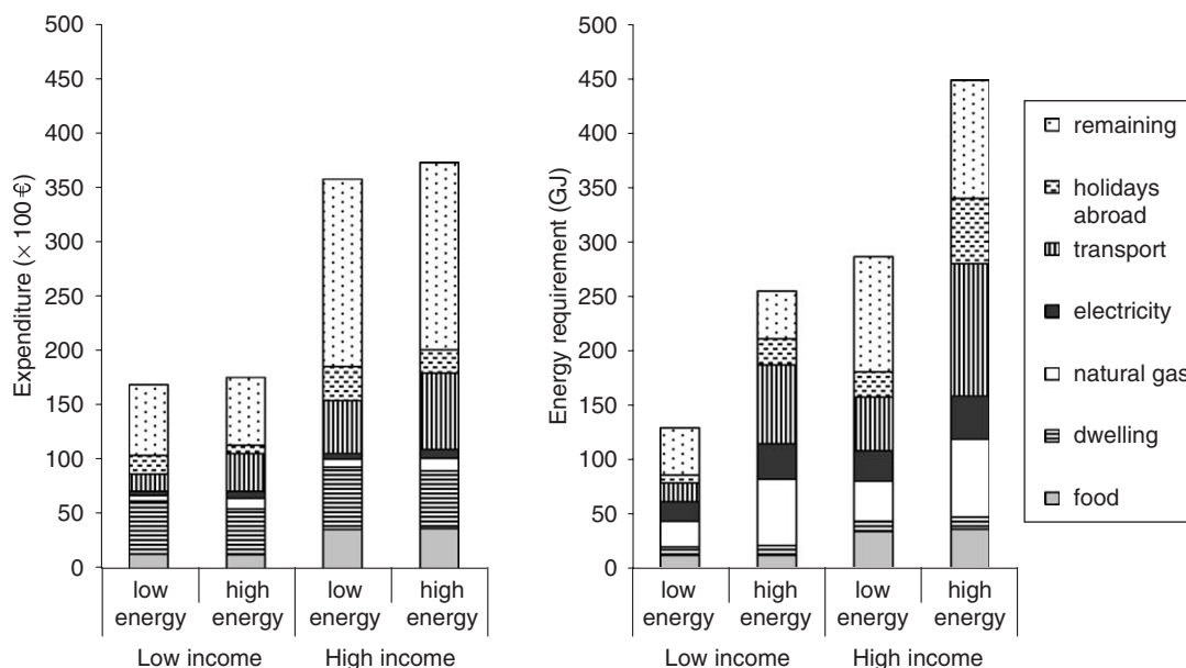
Fig. 7. Expenditures and energy requirement for low- and high-energy and for low- and high-income households.
