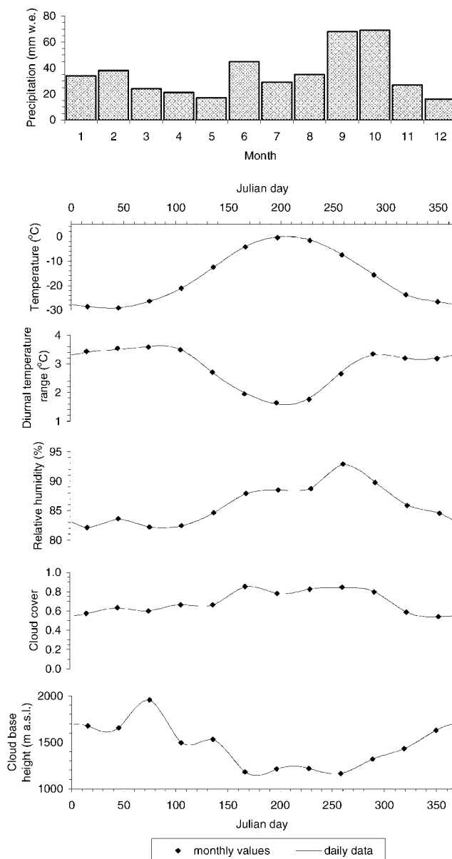
FIGURE 4. Monthly mean and daily meteorological data for the reference climate at Vavilov Station.
