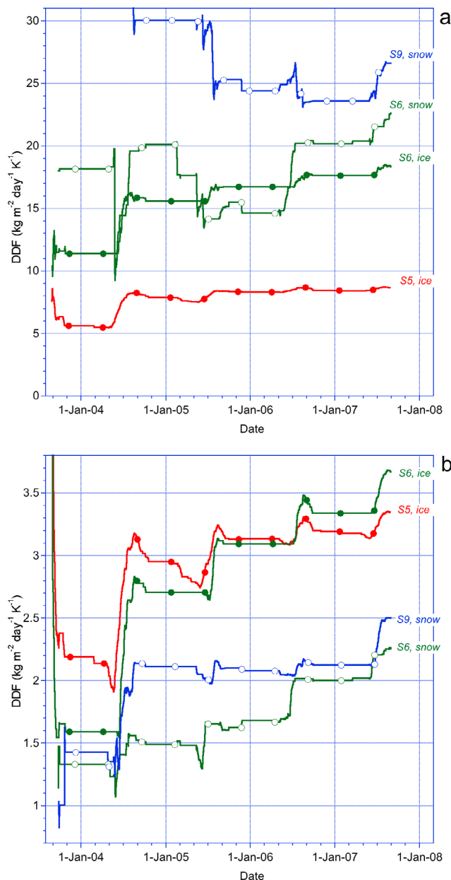
Figure 2. Cumulative Degree Day Factors for snow ( \text{DDF}_s , open symbols) and ice ( \text{DDF}_i , filled symbols) using the two threshold values of (a) T_0 = 273.15 \text{ K} and (b) T_0 = 268 \text{ K} . \text{DDF}_{i,s} are calculated using melt and positive degree-days cumulated up to that moment, which explains the decreasing variability in time. Note that no change in DDF occurs during winter, when the cumulative quantities do not change.
