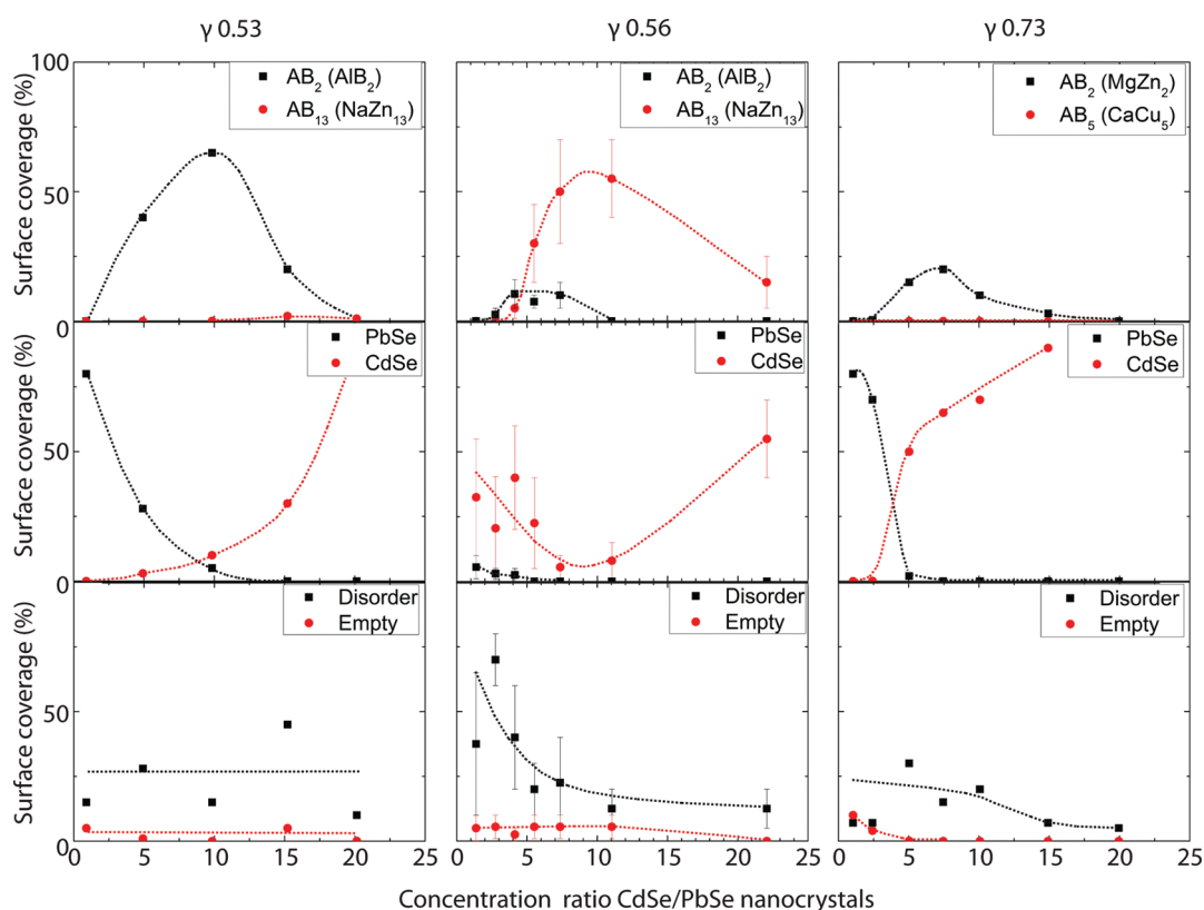
FIGURE 2. The effect of changing the particle concentration ratio in the binary mixtures on the relative importance of the formed single-component and binary NC superlattices. The size ratio of the large PbSe NCs with respect to the small CdSe NCs is \gamma = 0.53 (left panels), \gamma = 0.56 (center panels), and \gamma = 0.73 (right panels). The dotted lines are guides to the eye. The size ratio of 0.56 is from former published work. 11 The uncertainty on the % surface coverage is about 25 relative %.
