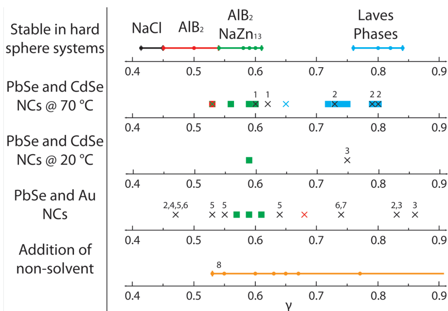
FIGURE 4. Schematic comparison of the structures that are experimentally observed with the theoretical phase diagrams for binary hard-sphere mixtures. Squares indicate crystal structures that are in agreement with the hard-sphere model. Crosses indicate crystal structures that are in disagreement with the hard sphere model: (1) refers to several unknown crystal structures (Supporting Information Figure SI3), coverage <1%; (2) PbSe(CdSe) 5 isostructural with CaCu 5 , coverage <1%, the coverage does not respond to a change in the composition; (3) CsCl structure; (4) NaCl structure; (5) CuAu structure; (6) Cu 3 Au structure. The crystal structures (1–6) have a low (~1%) surface coverage. The number 7 indicates the CsCl crystal structure, observed here with a surface coverage of about 30%. Number 8 is for the addition of a nonsolvent for which only single-component structures are observed.
