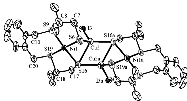
Figure 3. Displacement ellipsoid plot of [Ni(xbsms)CuI_2]_2 ( 2 ), drawn at the 50% probability level. Hydrogen atoms and solvent molecules have been omitted for clarity.
