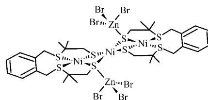
Figure 6. Proposed structure of [\text{Ni}_3(\text{xbsms})_2(\text{ZnBr}_3)_2] (4).
