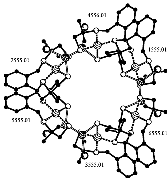
Figure 4. Stacking plot of [Ni(xbsms)CuI_2]_2 ( 2 ), including the ARU numbers. View along the 3_2 screw axis.
