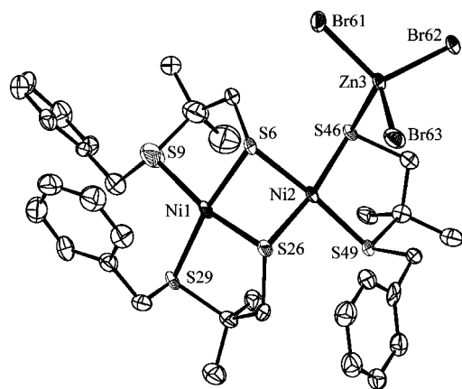
Figure 5. Displacement ellipsoid plot of [\text{Ni}_2(\text{bsms})_3\text{ZnBr}_3] (3), drawn at the 50% probability level. Hydrogen atoms and solvent molecules are omitted for clarity.
