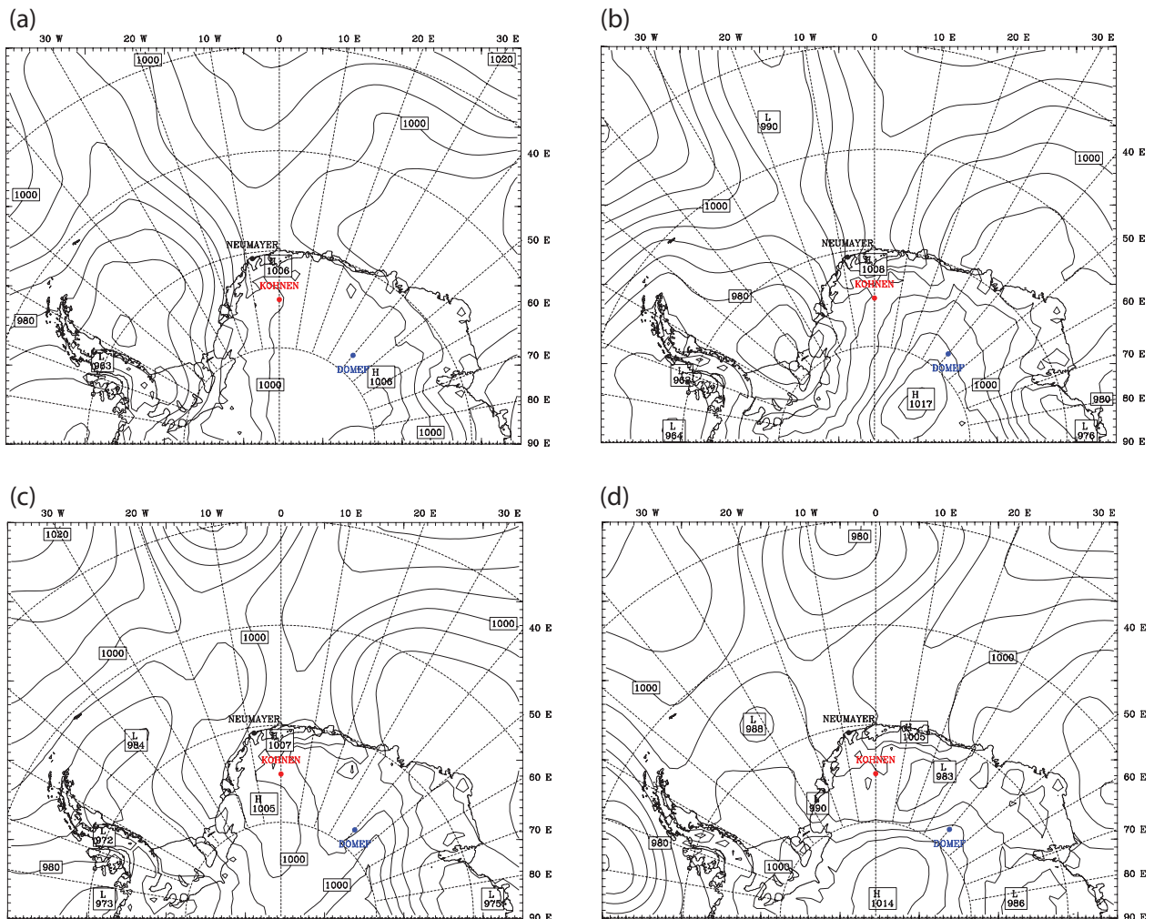
Fig. 3 Antarctic Mesoscale Prediction System surface pressure for (a) 22 February 2003, (b) 23 February 2003, (c) 24 February 2003 and (d) 25 February 2003; 12:00 GMT.
