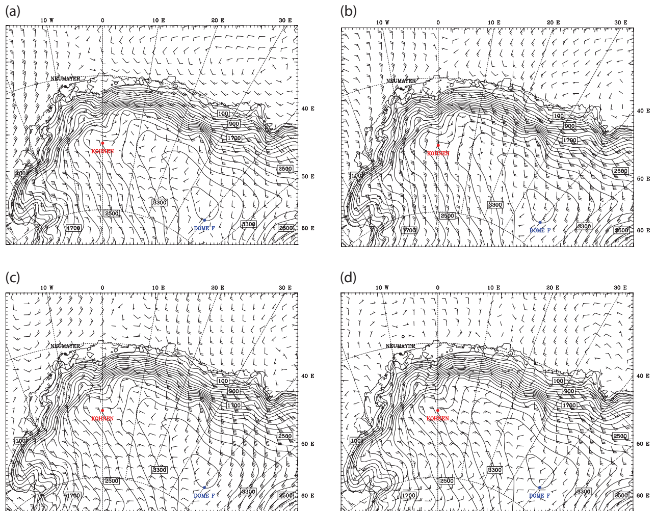
Fig. 5 Antarctic Mesoscale Prediction System surface winds for (a) 22 February 2003, (b) 23 February 2003, (c) 24 February 2003 and (d) 25 February 2003; 12:00 GMT.
