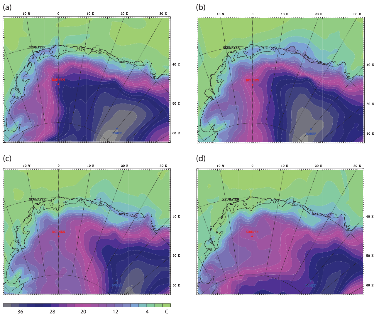
Fig. 8 Antarctic Mesoscale Prediction System surface temperature for (a) 22 February 2003, (b) 23 February 2003, (c) 24 February 2003 and (d) 25 February 2003; 12:00 GMT.
