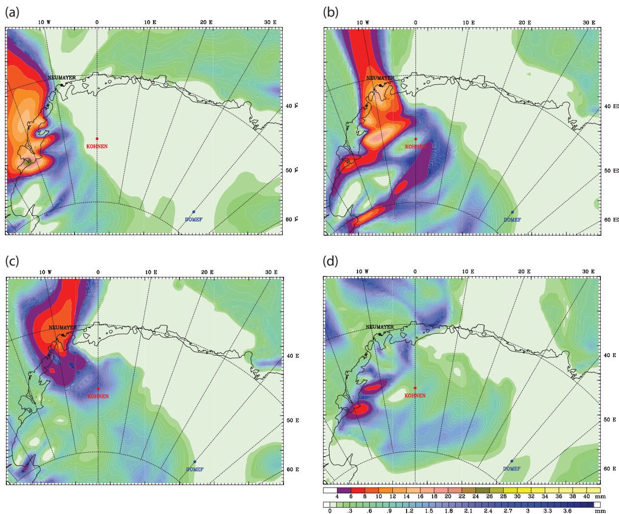
Fig. 6 Antarctic Mesoscale Prediction System precipitation for (a) 22 February 2003, (b) 23 February 2003, (c) 24 February 2003 and (d) 25 February 2003; 12:00 GMT.
