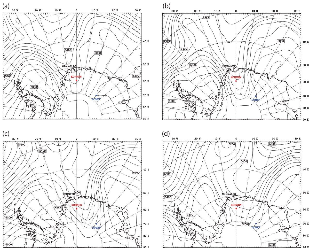
Fig. 4 Antarctic Mesoscale Prediction System 500-hPa geopotential height for (a) 22 February 2003, (b) 23 February 2003, (c) 24 February 2003 and (d) 25 February 2003; 12:00 GMT.
