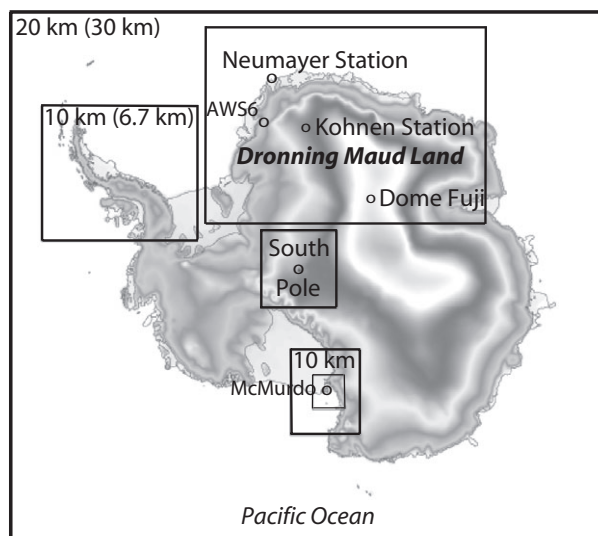
Fig. 1 Antarctic Mesoscale Prediction System grids: outer frame, 30-km domain (20 km since September 2005); 10-/6.7-km domains over Antarctic Peninsula, South Pole and western Ross Sea; 3.3-/2.2-km domain over Ross Island. An outer domain of 90/60 km (not shown) extends to New Zealand, Australia, South Africa and South America. Grey shades refer to model topography, which is shown in detail for Dronning Maud Land in Fig. 5. Locations mentioned in the text are also shown.
