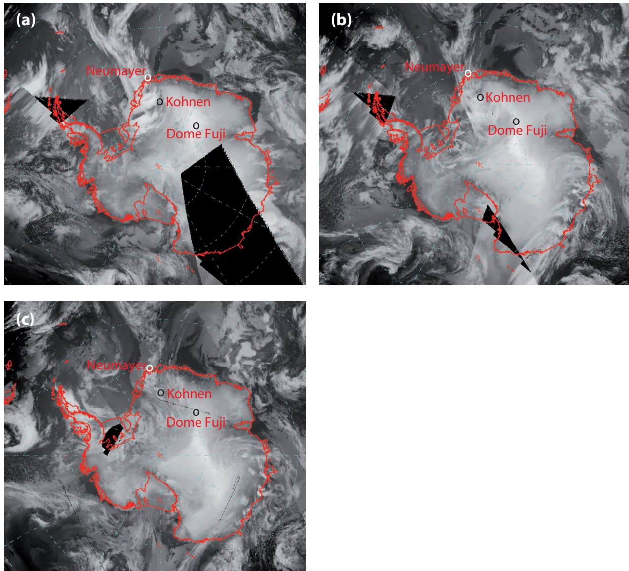
Fig. 7 Infrared composite satellite images for (a) 22 February 2003, (b) 23 February 2003, (c) 24 February 2003 and (d) 25 February 2003, 15:00 GMT.
