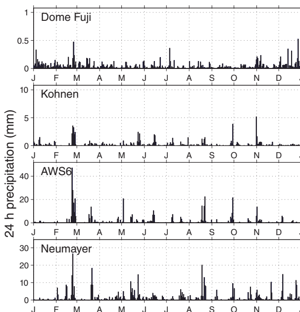
Fig. 2 Daily sums of precipitation for 2003 derived from the Antarctic Mesoscale Prediction System for Neumayer Station, AWS6, Kohnen Station and Dome Fuji.
