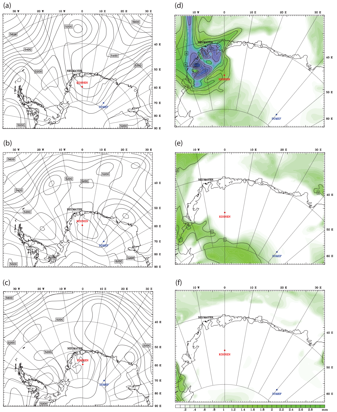
Fig. 12 Antarctic Mesoscale Prediction System 500-hPa geopotential height for 26 February at 12:00 GMT, 28 February at 12:00 GMT and 2 March 00:00 GMT, and Antarctic Mesoscale Prediction System 12-h precipitation sums for the corresponding 12-h time intervals following the dates above.
