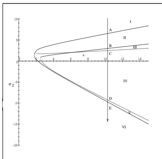
FIGURE 13. The parameter diagram of system (4.1) in the (a, \sigma_2) -plane for c_2 < 0
