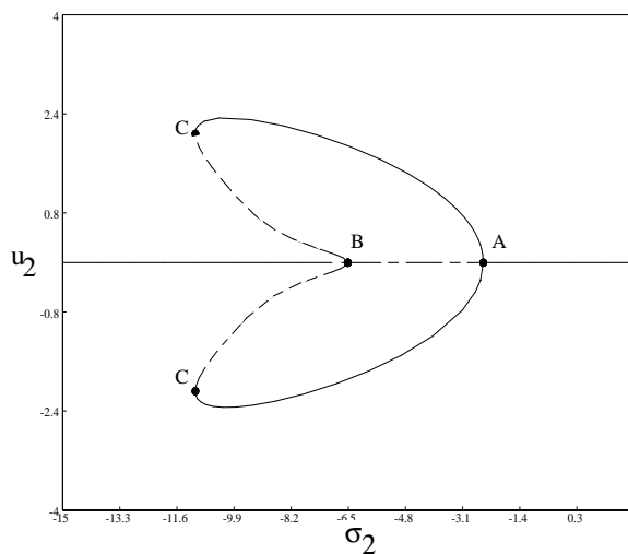
FIGURE 8. The bifurcation diagram of the semi-trivial solution in the (\sigma_2, u_2) -plane for c_2 > 0 .
