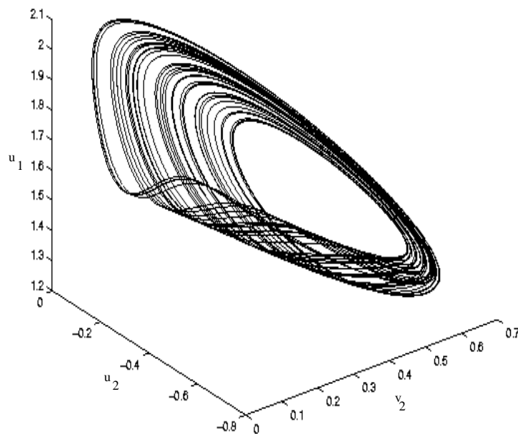
FIGURE 18. The strange attractor of the averaged system (2.5). The phase-portraits in the (u_2, v_2, u_1) -space for c_2 < 0 at the value \sigma_2 = 5.3 .
