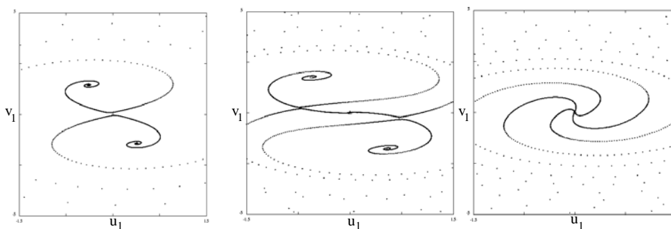
FIGURE 2. The phase-portraits of system (3.1) in the (u_1, v_1) -plane for specific values (\sigma_1, a) in region I, II, and III, respectively.
