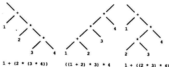
Figure 5: Three trees representing the expression 1 + 2 * 3 * 4 , based on the ambiguous grammar of Figure 2
