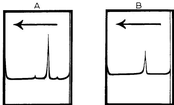
Fig. 3. Ultracentrifuge patterns of two preparations of microsomal RNP particles at different stages of the purification procedure. A. A rather crude preparation (see text) in a solution containing: 0.0025 M K 2 HPO 4 , 0.0025 M KH 2 PO 4 , 0.001 M MgSO 4 ·H 2 O, 7.5·10 -4 M CaCl 2 . Speed: 42,040 r.p.m., bar angle 45°, after 13 minutes of sedimentation. B. A final preparation in the same solution. Speed: 42,040 r.p.m., bar angle 40°, after 14 minutes of sedimentation.
