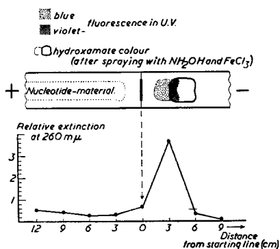
Fig. 1. Schematic outline of an electrophoresis experiment with the concentrated dialysate, showing the coincidence of the hydroxamate-forming material with a peak in the 260 \text{m}\mu absorption. Electrophoresis at 10 \text{V cm}^{-1} for 16 hours in 0.02 M citrate buffer, pH 3.9.
