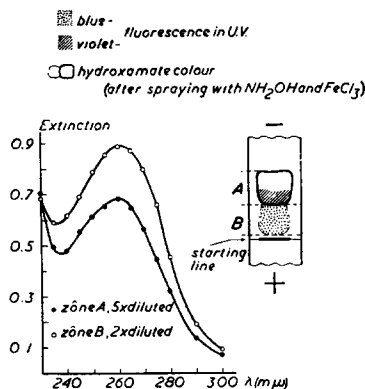
Fig. 2. U.V.-absorption spectra in 0.05 M phosphate buffer (pH 6.8) of the hydroxamate-forming material as obtained after an electrophoresis experiment for 16 hours at 10 \text{V cm}^{-1} in 0.02 M citrate buffer, pH 3.9.
