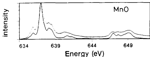
Fig. 3. Manganese 2p X-ray absorption spectrum of MnO (dotted) compared with a crystal field multiplet calculation (solid line). A crystal field strength of 0.8 eV was used.
