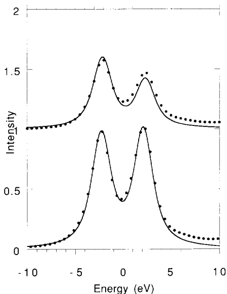
Fig. 1. Comparison of a crystal field multiplet calculation of \text{Mo}^{6+} , 4d^0 (solid line) with an experimental spectrum of gaseous \text{MoF}_6 (points). The L_2 edge (top) and the L_3 edge (bottom) have been aligned. A crystal field strength of 4.5 eV was used.
