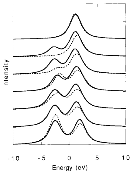
Fig. 2. Crystal field multiplet calculations for molybdenum. The L_3 edge (solid line) and the L_2 edge (dashed) are given for 4d^0 (bottom), 4d^1 , 4d^2 , 4d^3 , 4d^4 , 4d^5 and 4d^6 (top) ground state configurations. Crystal field strengths of 4.0 eV were used.
