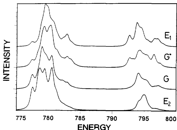
Fig. 4. Crystal field multiplet calculations for the transition from a high-spin 3d^7 state as present in CoO. The spectra of the four spin-orbit split configurations are shown. A crystal field strength of 0.8 eV was used.
