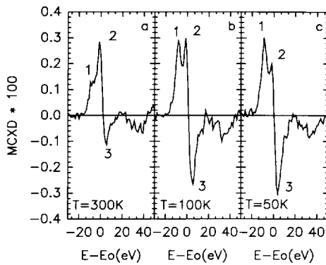
Fig. 1. MCXD at L_3 edge of Yb in \text{YbFe}_2 for \alpha = 0^\circ at (a) T = 300\text{ K} , (b) T = 100\text{ K} , (c) T = 50\text{ K} .
