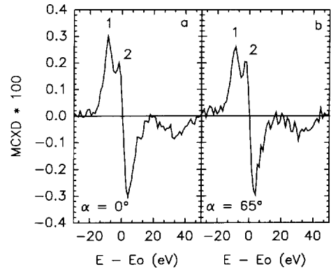
Fig. 2. MCXD at L_3 edge of \text{YbFe}_2 at T = 50\text{ K} , (a) \alpha = 0^\circ , (b) \alpha = 65^\circ [normalised by \cos(65^\circ) ].
