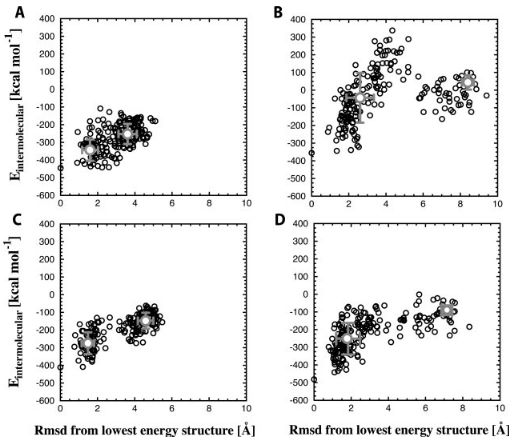
Fig. 1. Intermolecular energies ( E_{vdw} + E_{elec} + E_{restraints} ) versus backbone RMSD from the lowest-energy structure. Values for single structures are indicated by black dots, and cluster averages and standard deviations are shown in gray: (a) CSP, (b) VEAN, (c) SANI, and (d) final protocol, VEAN-SANI. For a description of the different docking runs, see text and footnote e of Table II.
