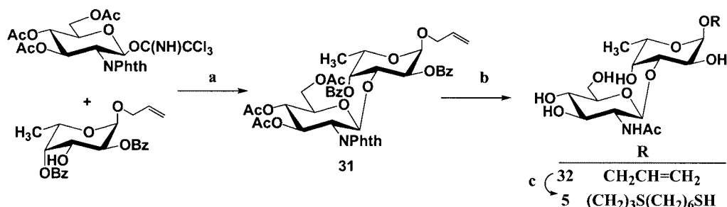
Scheme 5. Reagents and conditions. a, acceptor, donor, TMSOTf, \text{CH}_2\text{Cl}_2 , 86%. b, (i) ethylenediamine, n BuOH, 90 °C; (ii) acetic anhydride, pyridine; (iii) NaOMe, MeOH, 80% over three reaction steps. c, 1,6-hexanedithiol, UV light, MeOH, quantitative. (Bz = \text{COC}_6\text{H}_5 )
