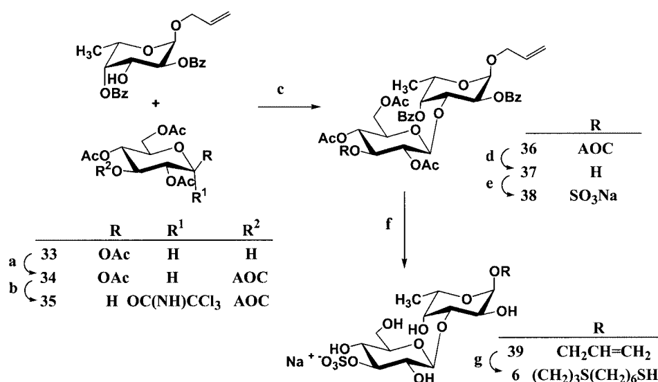
Scheme 6. Reagents and conditions. a, allyl chloroformate, pyridine, \text{CH}_2\text{Cl}_2 , -30 °C, quantitative. b, (i) \text{NH}_2\text{NH}_2\cdot\text{HOAc} , DMF; (ii) trichloroacetonitrile, 1,8-diazabicyclo[5.4.0]undec-7-ene, \text{CH}_2\text{Cl}_2 , 60% over two reaction steps. c, donor 35 , acceptor, TMSOTf, \text{CH}_2\text{Cl}_2 , 60%. d, [\text{Pd}(\text{PPh}_3)_4] , morpholine, THF, 65 °C, 93%. e, \text{SO}_3\cdot\text{NMe}_3 , DMF, 50 °C, 53%. f, NaOMe, MeOH, quantitative. g, 1,6-hexanedithiol, UV light, MeOH, 50%. (AOC = \text{COOCH}_2\text{CH}=\text{CH}_2 ; Bz = \text{COC}_6\text{H}_5 )
