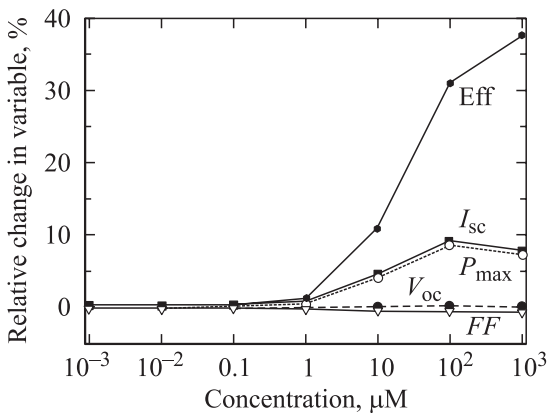
Figure 8. The relative change of the variables I_{sc} , V_{oc} , FF , P_{max} , and efficiency (Eff) of the mc-Si solar cell as a function of QD concentration.
