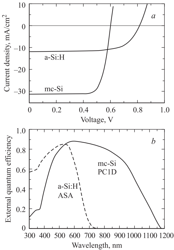
Figure 2. Performance of the two solar cells, mc-Si and a-Si:H: a — current-voltage characteristics; b — spectral response.
