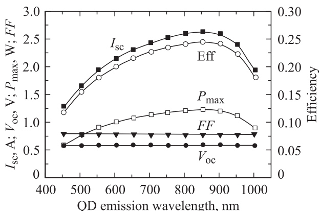
Figure 5. Effect of small-band QD emission (500 W/m 2 ) on the parameters I_{sc} , V_{oc} , FF , P_{max} , and efficiency (Eff) of the mc-Si solar cell as a function of center emission wavelength. Left-hand scale: I_{sc} , V_{oc} , and P_{max} ; right-hand scale — efficiency.
