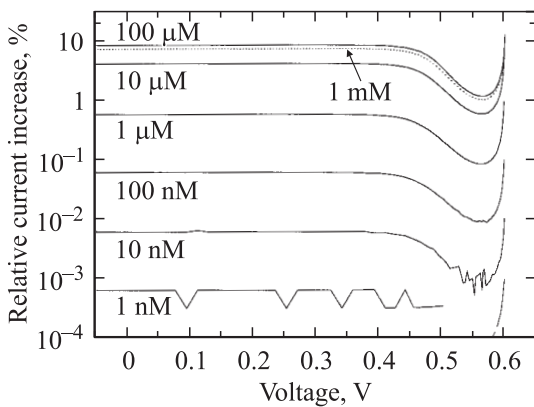
Figure 7. The effect of QD concentration on the current of the mc-Si solar cell as a function of cell voltage, shown as the current increase relative to the base case (AM1.5G).
