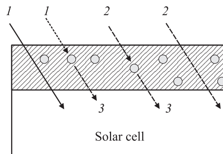
Figure 1. Schematic drawing of the studied configuration. A plastic layer containing quantum dots is applied on top of a solar cell. Both blue (1) and green (2) light are absorbed by the quantum dot and re-emitted in the red (3), which is subsequently absorbed in the solar cell. Also, unabsorbed blue and green light enters the solar cell as well.
