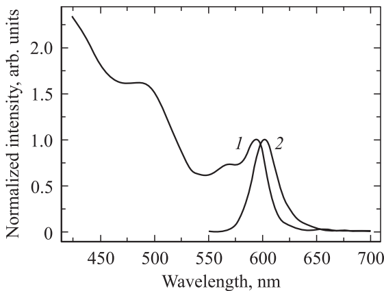
Figure 3. Normalized absorption (1) and emission (2) spectrum of CdSe nanocrystals of 4.3 nm diameter, capped with TOPO/TOP/HDA (data from S.F. Wuister (2003), see also Ref. [30]).
