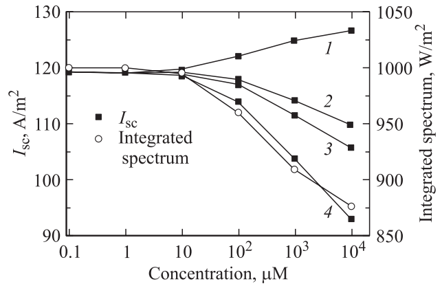
Figure 9. The relative change of the short-circuit current I_{sc} of the a-Si:H solar cell as a function of QD concentration for combinations of the quantum efficiency \eta_e and capture efficiency \eta_t : 1 — \eta_e = 1 , \eta_t = 1 , 2 — \eta_e = 0.8 , \eta_t = 1 , 3 — \eta_e = 1 , \eta_t = 0.75 , and 4 — \eta_e = 0.8 , \eta_t = 0.75 . The integrated spectrum is shown to the right-hand scale for \eta_e = 0.8 , \eta_t = 0.75 .
