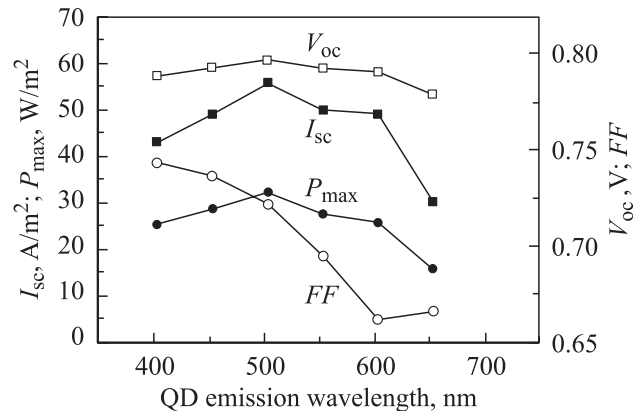
Figure 6. Effect of small-band QD emission (500 W/m 2 ) on the parameters I_{sc} , V_{oc} , FF , and P_{max} of the a-Si:H solar cell as a function of center emission wavelength. Left-hand scale: I_{sc} and P_{max} ; right-hand scale: V_{oc} and FF .
