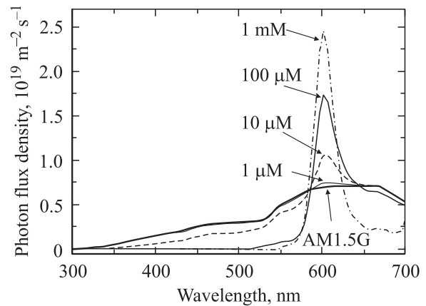
Figure 4. Calculated modified spectra for various molar QD concentrations that notably influence the AM1.5G spectrum, i.e., 1, 10, and 100\ \mu\text{M} and 1 mM.
