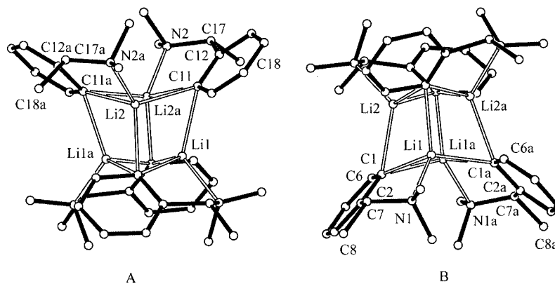
Figure 1. Ball-and-stick model of ( R )- 2 in two different orientations; rotation (90°) of A along the y axis gives B; the C 2 dimeric unit is clearly visible in the upper half of the Li 4 tetrahedron of A, while the C 1 dimeric unit can be seen in the lower half of B (for C 1 and C 2 , see Figure 4)
