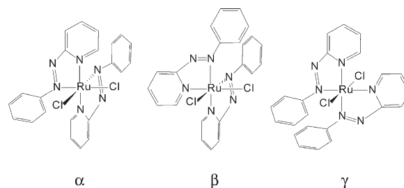
Fig. 1 Schematic representation of the three most common isomers of the [Ru(azpy) 2 Cl 2 ] complexes: the \alpha isomer with the coordinating pairs N py trans , N azo cis and Cl cis (left), the \beta isomer with the coordinating pairs N py cis , N azo cis and Cl cis (middle) and the \gamma isomer with the coordination pairs N py cis , N azo cis and Cl trans (right).
