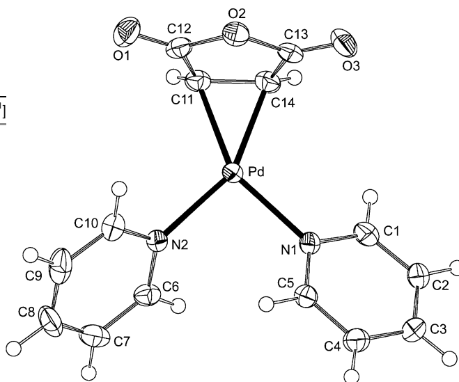
Figure 1. Displacement ellipsoid plot (50% probability level) of compound 1 . Selected distances [ \text{\AA} ] and angles [ ^\circ ]: Pd-N1 2.1472(19), Pd-N2 2.1462(18), Pd-C11 2.068(2), Pd-C14 2.062(2), C11-C14 1.430(3), C11-Pd-C14 40.51(10), N1-Pd-N2 94.44(7), C11-Pd-N1 151.96(9), C14-Pd-N2 153.81(8), C11-Pd-N2 113.32(9), C14-Pd-N1 111.73(8), Pd-C11-C12 108.29(17), Pd-C14-C13 105.07(17).
