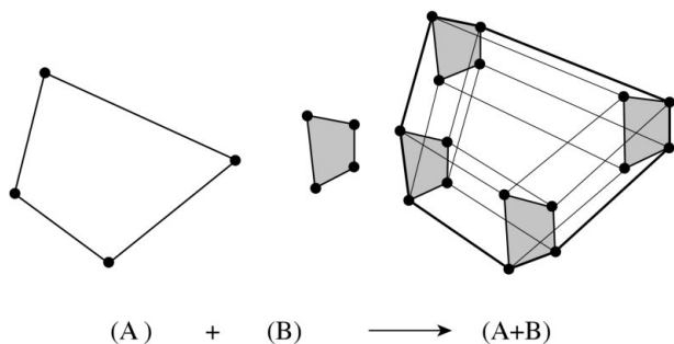
Figure 8 Adding the contours A and B by translating B along the edges of A . This method is applied repeatedly to construct a complete reflection from the calculated sub-reflections.
