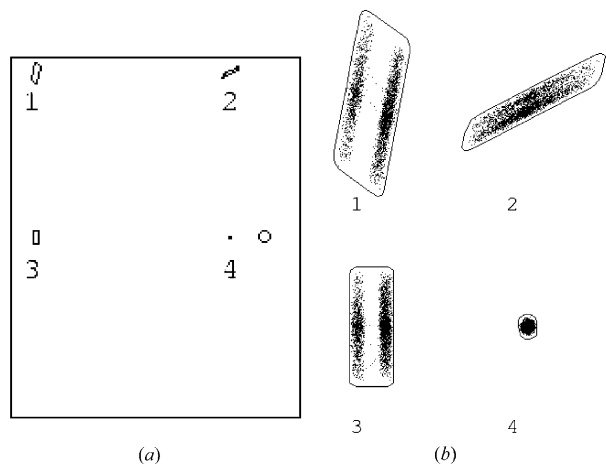
Figure 10 (a) Schematic representation of the whole detector with the predicted X_D Y_D reflection contours for one and the same crystal but for different reflections, impacting at four indicated positions. ‘o’ is the primary beamstop. Parameters: focus 0.3 \times 3 mm at 220 mm, take-off angle 5.7^\circ , \lambda_1 = 0.7093 , \lambda_2 = 0.7136 Å, detector distance 40 mm, swing = -35^\circ , spherical crystal diameter 0.2 mm, mosaicity 2^\circ . (b) The same reflections equally magnified. Note the \alpha_1 – \alpha_2 splitting, especially in reflections 1 and 3. The specks within each contour are some calculated random impacts. Results: reflection size (closest surrounding box x_D \times y_D \times \omega ): (1) 1.52 mm \times 3.66 mm \times 2.83^\circ ( \theta = 37.19^\circ ); (2) 2.84 mm \times 1.92 mm \times 13.60^\circ ( \theta = 16.47^\circ ); (3) 0.88 mm \times 2.36 mm \times 2.58^\circ ( \theta = 35.94^\circ ); (4) 3.10 mm \times 0.35 mm \times 2.14^\circ ( \theta = 3.10^\circ ). Reflection 2 (which would extend over 27 images if \Delta\omega where 0.5^\circ , as in Fig. 11) is a typical example of a reflection that could well be rejected by EVAL-14 by the rule |\chi| + \theta < 90^\circ - \Delta (see §6).
