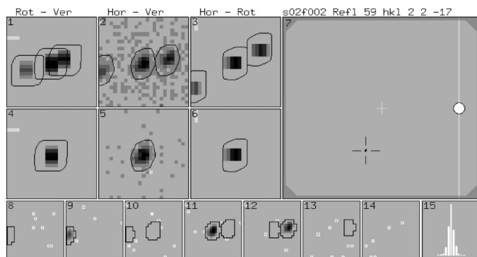
Figure 11 EVAL-14 at work on a twin lattice. Windows 8 through 14 show the primary data: seven slices each of 25 \times 25 pixels with a \Delta\omega depth of 0.5^\circ , forming the shoe box. The central contours in windows 10, 11 and 12 are the expected contours of the main reflection in those slices; the two (stronger) reflections extending over windows (8, 9, 10) left and (11, 12, 13) right are intruders from a twin lattice, falling neatly within their expected contours. Windows 1, 2 and 3 are the y_D \omega , x_D y_D and \omega x_D projections, respectively, of the complete shoe box. The row 4, 5 and 6 gives the final results: the aliens are eliminated and the BPB method can be applied successfully. Window 7 shows the complete detector with the position of the reflection under consideration (open black cross), detector centre (white cross) and primary beam impact (white circle); window 15 gives the net \omega reflection profile. For details of the lattices see the work by Lutz et al. (1999).
