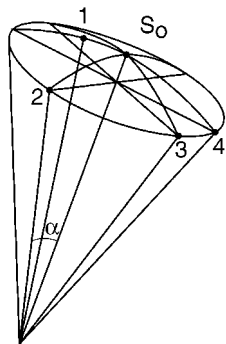
Figure 4 Mosaicity model. \mathbf{S}_0 is the central reflection vector \mathbf{S}_0(h,k,l) . With isotropic mosaicity the mosaic vectors \mathbf{S}_m ( |\mathbf{S}_m| = |\mathbf{S}_0| ) form a massive circular cone around \mathbf{S}_0 , with 2\alpha = \mu , the full mosaicity. 1 represents a general \mathbf{S}_m vector; 2, 3 and 4 are special ('extreme') \mathbf{S}_{m,E} vectors on the cone mantle. With anisotropic mosaicity the circular domain through ( 2, 3, 4 ) is elliptically stretched.
