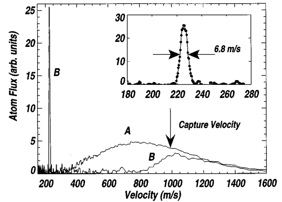
FIG. 3. Measured velocity distributions both with and without the slowing laser beam. The curve labeled A indicates the unslowed distribution from the source. Curve B shows the distribution after slowing. The arrow indicates the maximum of the velocity capture range of the slowing laser. The inset shows an enlarged portion of the figure in which the strong collection of atoms at low velocities is clearly visible.
