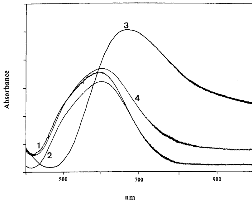
FIG. 1. DRS spectra of [\text{Cu}(\text{lysine})_2]^{2+} -saponite materials (CULYS2) after different treatments: (1) as prepared; (2) dried at 50^\circ\text{C} ; (3) after ammonia adsorption; and (4) after ammonia desorption.
