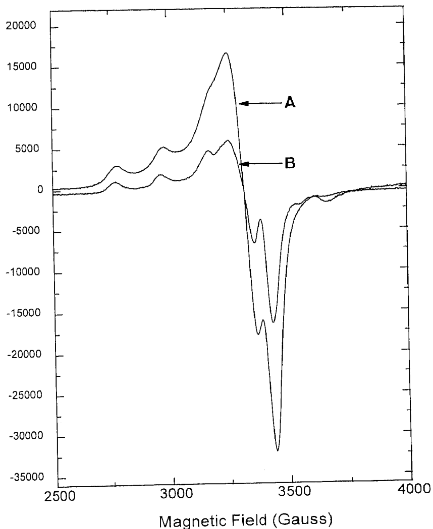
FIG. 2. ESR spectra of [\text{Cu}(\text{AA})_2]^{2+} -saponite: (A) CULYS2 and (B) CUHIS2.
