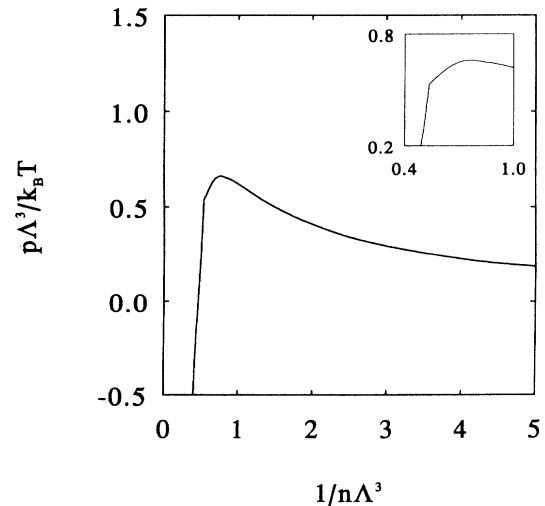
FIG. 2. Pressure as a function of inverse density for a fixed temperature such that |a/\Lambda| = 10^{-1} . The inset shows the cusp in the pressure caused by the Evans-Rashid transition.
