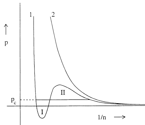
FIG. 1. Qualitative picture of the relationship between pressure and inverse density at a fixed and sufficiently low temperature for (1) atomic lithium or cesium and (2) atomic hydrogen. Note that possible cusps in the curves due to symmetry-breaking phase transitions are not shown here.
