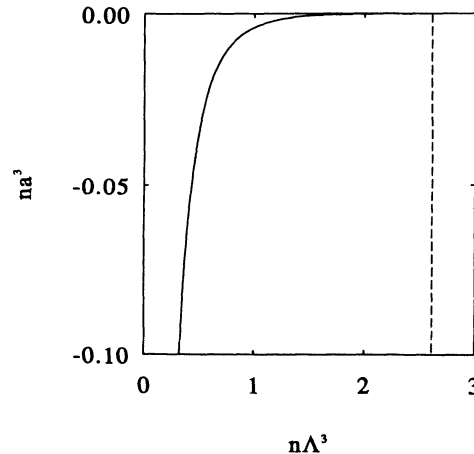
FIG. 3. Spinodal line in the (n\Lambda^3, na^3) plane, separating the (meta)stable and unstable regions of the phase diagram. The dashed line corresponds to the condition for Bose-Einstein condensation in a Bose gas with repulsive interactions.
