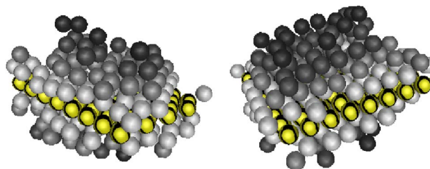
FIG. 3. (Color online) Snapshots of 111 (left-hand side) and 100 (right-hand side) templates. The particles that belong to the template have been highlighted by a black circular border. The grey spheres represent solid particles crystallizing directly on the template. Darker grey labels represent crystalline particles in subsequent layers.
