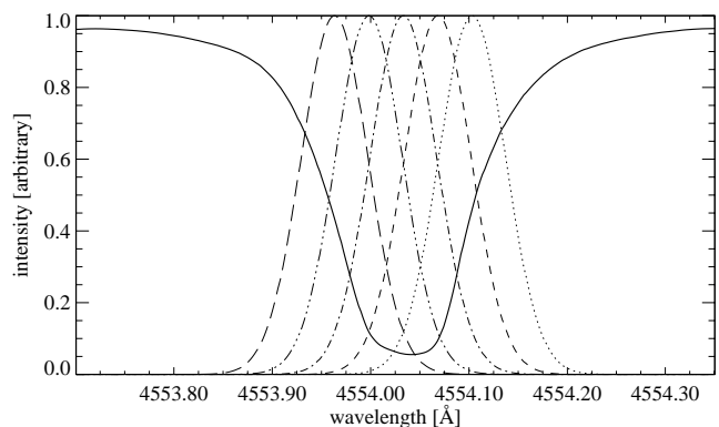
Fig. 3. Spatially-averaged disk-center profile of the Ba II 4554 Å resonance line taken from Neckel (1999). The five tunable-filter band-passes used in this paper are superimposed assuming a Gaussian band-pass shape.
