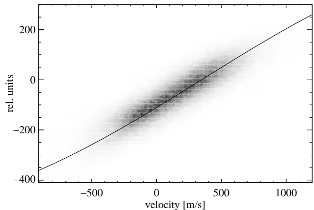
Fig. 7. Scatter plot of two-point intensity differences as defined by Eq. 1 (vertical) against five-wavelength Dopplershift measurement (horizontal) per pixel. The curve shows the relation expected from the mean disk-center profile and the bandpass shape shown in Fig. 3.
