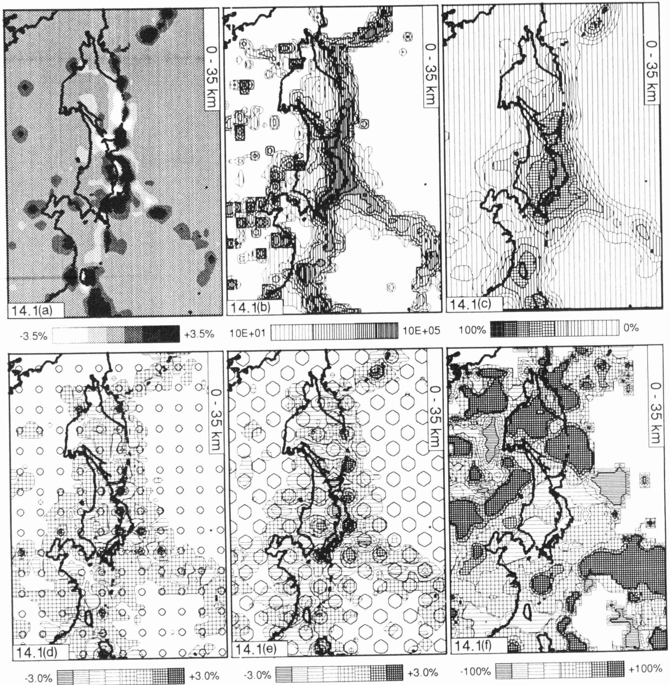
Figure 14. Inversion results for lithosphere, upper mantle, and transition zone layers of the block model (see text Section 4.1 for a detailed explanation). The numbers [1–11] correlate to the layer numbers in Table 1. (a) [1–11] Solution of the inversion for aspherical Earth structure. Velocity perturbations relative to iasp91 are contoured in seven intervals between -3.5 and +3.5 per cent ( cf. Section 4.1.1). (b) [1–11] Sampling of structure. Number of rays that sample blocks of the cell model (hit count, cf. Section 4.1.2). The scale is logarithmic. (c) [1–11] Resolution test. Fit between checker board-type input model and inversion response ( cf. Section 4.1.5). A value of 0 per cent indicates that the input structure is not resolved. A value of 100 per cent would indicate perfect recovery of input structure. (d) [1–11] Resolution test. Inversion response to the block anomaly model ( cf. Section 4.1.3). (e) [1–11] Resolution test. Inversion response to the harmonic anomaly model ( cf. Section 4.1.4). (f) [1–11] Effect on resolution of incorporating pP -wave ray paths ( cf. Section 4.1.6). The values are given with respect to the model fit obtained with P -wave ray paths only ( cf. Section 4.1.5).
