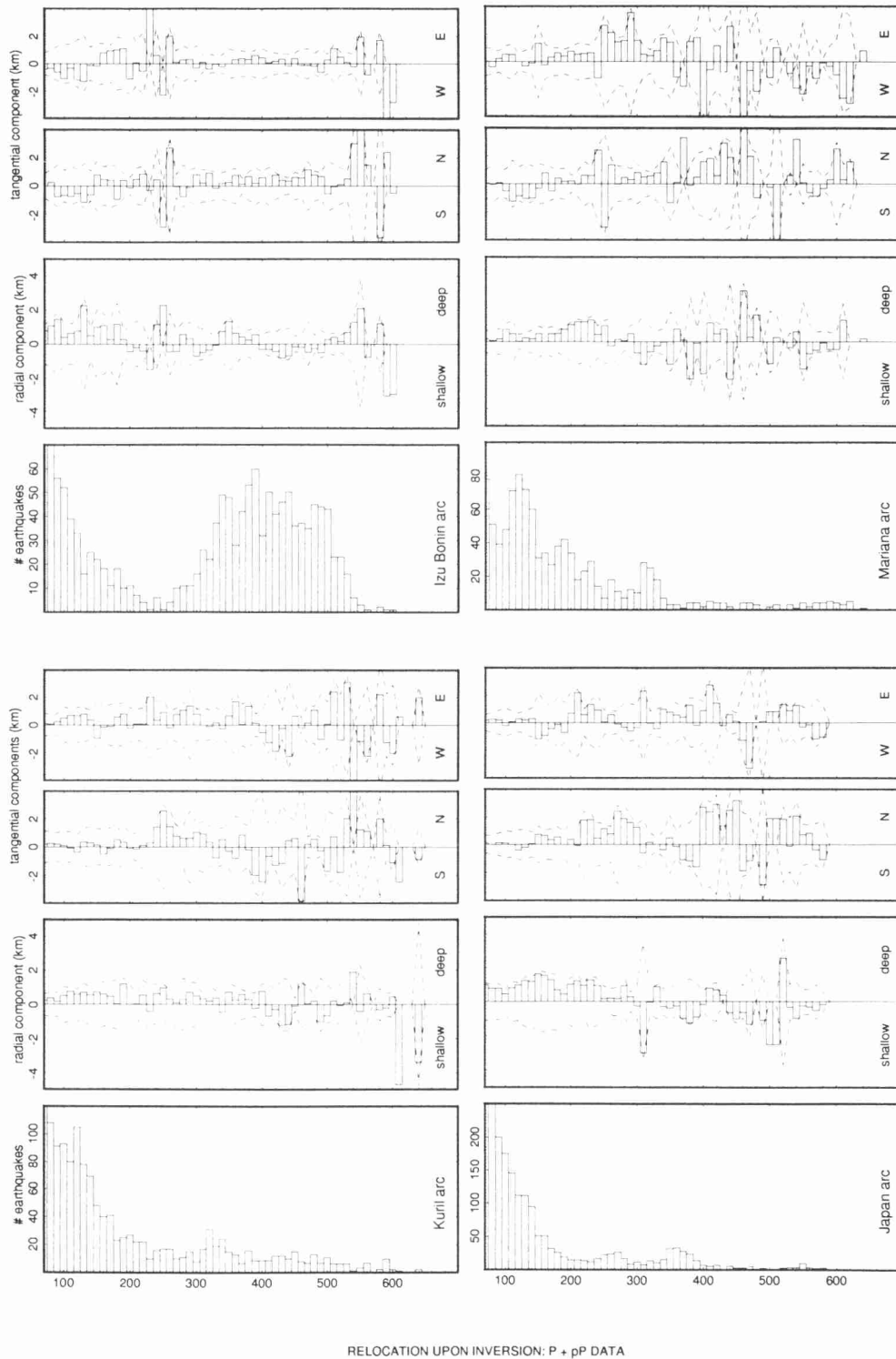
Figure 16. Spatial components of the relocation vectors for earthquakes in four major seismic zones of the northwest Pacific region. The relocation vectors are determined upon inversion of P and pP traveltime residuals for 3-D Earth structure. For each of the seismic zones the depth distribution of seismicity is given in the leftmost panel; the depth relocation (radial component) and epicentre relocation (tangential components) averaged over 10 km depth bins are presented in the other two panels. Dashed lines are drawn at \pm\frac{1}{2}\sigma , where \sigma is the standard deviation of the average relocation in a particular depth bin. We refer to Van der Hilst & Engdahl (1992) for a detailed discussion.
