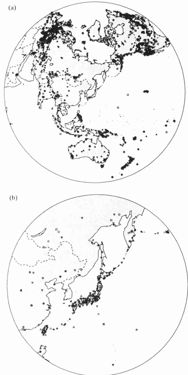
Figure 6. Distribution of the seismicological stations that contributed to the data set used in our inversion. (a) Seismological stations located outside the study region. (b) Stations located within the study region.
