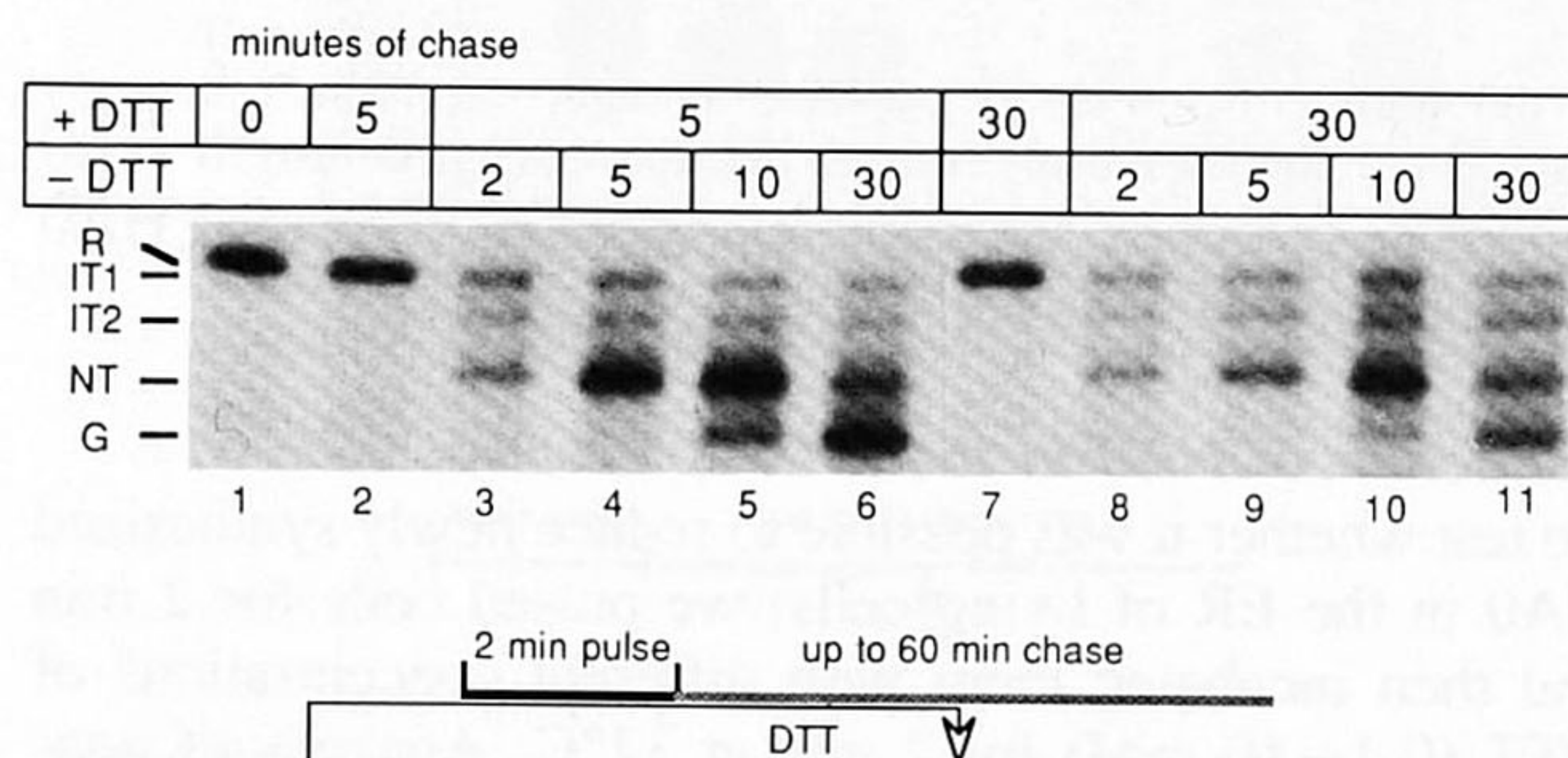
Fig. 4. Post-translational folding of HA0 translated in the presence of 5 mM DTT. The experimental protocol was as in Figure 2A, except that 5 mM DTT was also present during and 5 min before the pulse. Long exposures were used for photographs. On shorter exposures, a precursor-product relationship between IT1, IT2 and NT has been established before (Braakman et al. , 1991).
