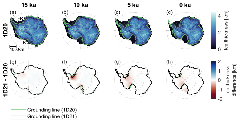
Figure 6. Ice thickness of 1D20 (a–d) and the difference in ice thickness between 1D20 and 1D21 (e–h) at four epochs during the deglaciation phase. (a) FR refers to the Filchner–Ronne Ice Shelf and R refers to the Ross Embayment. In panels (e)–(h), the 1D20 grounding line (green) mostly overlaps with the 1D21 grounding line (black).
