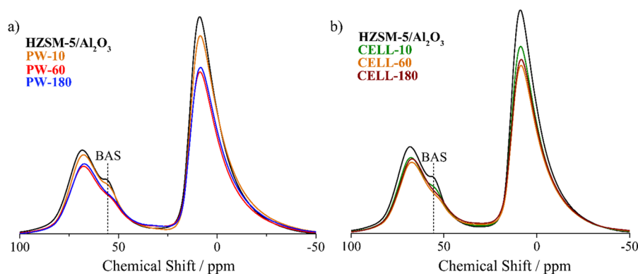
Figure 8. 27 Al solid state nuclear magnetic resonance (ss-NMR) spectra of (a) spent extrudates obtained after catalytic fast pyrolysis (CFP) of pine wood and (b) spent extrudates obtained after CFP of cellulose.
