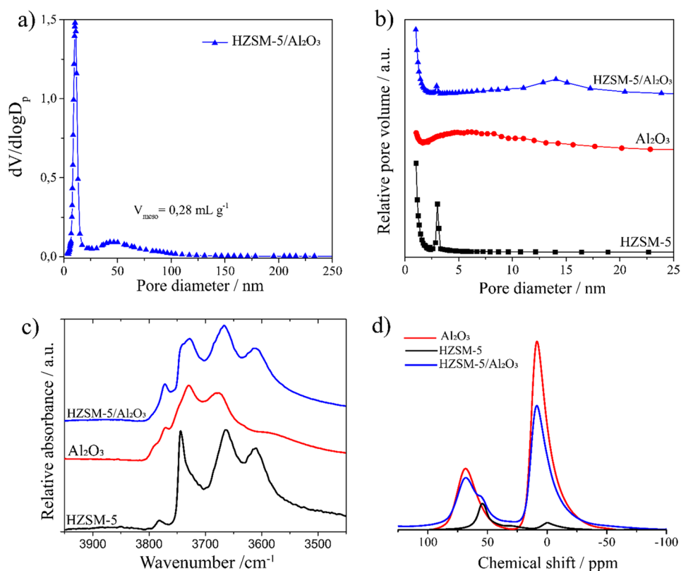
Figure 1. Pore size distribution graphs after (a) Hg porosimetry and (b) Ar physisorption at -196\text{ }^{\circ}\text{C} . (c) Fourier transform-infrared (FT-IR) spectra of the OH-stretching region. (d) ^{27}\text{Al} solid state nuclear magnetic resonance (ss-NMR) of fresh, individual components and the HZSM-5/ \text{Al}_2\text{O}_3 catalyst extrudates. The intensities in the ss-NMR spectra were normalized by weight.
