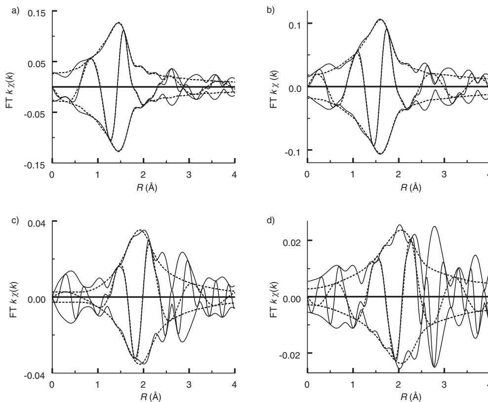
Figure 5. Fourier transforms ( k^1 , \Delta k=3-13 \text{ \AA}^{-1} ) of difference files (solid lines) and fits (dotted lines) of a) Cr-O, b) Cr-N, c) Cr-Cl, and d) Cr-C.
