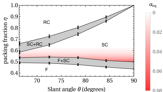
FIG. 8. Phase diagram in the \theta - \eta plane for the slanted cube system. Indicated are the fluid (F), simple cubic crystal (SC), and rhombic crystal (RC) phases. The gray shaded areas denote coexistence regions, and the (red) colouring represents the equilibrium vacancy concentration in the SC phase. The lines connect the points and merely serve to guide the eye.
