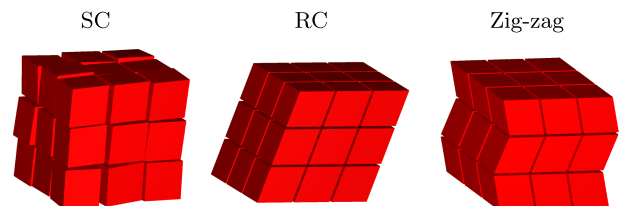
FIG. 3. Likely candidate crystal structures for the slanted cube particle shape. From left to right: a plastic simple cubic crystal, a rhombic crystal, and a zig-zag crystal.
