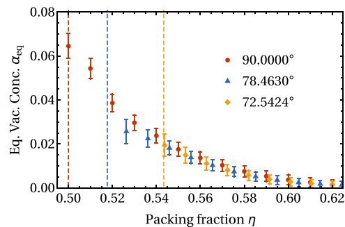
FIG. 7. The equilibrium vacancy concentration \alpha_{\text{eq}} as a function of the packing fraction \eta . The dashed lines indicate the melting densities. The equilibrium vacancy concentration is independent of the slant angle when compared at the same packing fraction.
