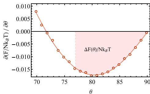
FIG. 2. Typical example of the behavior of the derivative \partial F/\partial\theta (in dimensionless units of k_B T per particle) in a defect-free simple cubic crystal of slanted cubes at a density \rho\sigma^3 = 0.58 . The solid line is a polynomial fit through the data points, and the shaded area corresponds to the free-energy difference \Delta F(\theta) = F(90^\circ) - F(\theta) .
