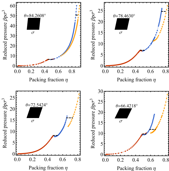
FIG. 4. Equations of state for various slant angles. For all slant angles, we find three phases. Namely, at low densities, a fluid (red); at intermediate densities, a simple cubic crystal phase (blue); and at high densities, a rhombic crystal phase (yellow). Dashed black lines indicate the coexistence densities and pressure as determined by free-energy calculations.
