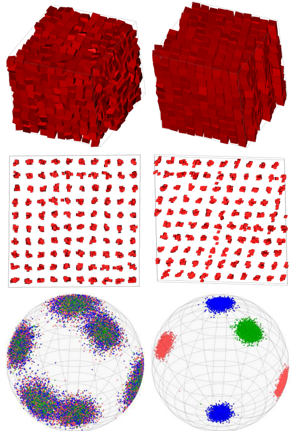
FIG. 5. Crystal phases of slanted cubes. Top row: snapshots with particles depicted at their true size. Middle row: particles shrunk to a fraction of their true size to show the crystal lattice. Bottom: scatter plot of the particle orientations. Red, green, and blue indicate, respectively, the \hat{x} , \hat{y} , and \hat{z} unit vectors in the reference frame of the particle (Fig. 1). The left column shows the simple cubic crystal phase and the right column shows the rhombic crystal phase.
