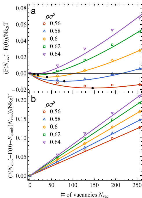
FIG. 6. (a) Fits through the vacancy contributions to the free energies of an SC crystal of slanted cubes with a slant angle \theta = 78.463^\circ with N_L = 8000 lattice sites. The fitted value for F(0) has been subtracted to plot all curves in the same graph. Open symbols indicate the data, solid lines indicate the fits, and filled (black) symbols indicate the minimum of these fits: the equilibrium vacancy concentration. (b) The same as top, but with the combinatorial term subtracted as well. The linear dependence on the number of vacancies can be seen clearly here.
