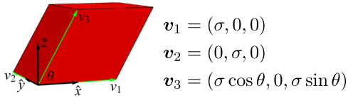
FIG. 1. A slanted cube with edge length \sigma and slant angle \theta .
