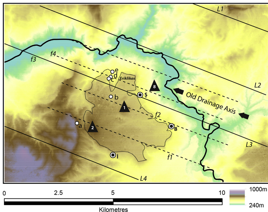
Fig. 8. Close-up view of the 10 m DEM in the area around the İbrahimğa plateau. Locations a-e represent outcrops described in the text. Lineaments L1-L4 are those identified in Fig. 7. Dotted lines, together with lineament L3 represent faults (f1-f4): f1-f3 are identified using offset of the Ulubey Fm. and fault f4 is identified at outcrop d.
