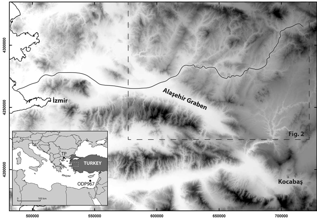
Fig. 1. General location of the study area in Western Anatolia, Turkey. Inset shows location of Turkey within the Mediterranean Basin. TP is Tenaghi Philippon. Also shown is location of ODP967 (Kroon et al., 1998). Dashed box shows approximate location of Fig. 2. Background image is the ASTER Global Digital Elevation Model (GDEM; ASTER GDEM is a product of METI and NASA) with heights ranging from 0 to 2400 m. Grid is in UTM Zone 35 coordinates.
