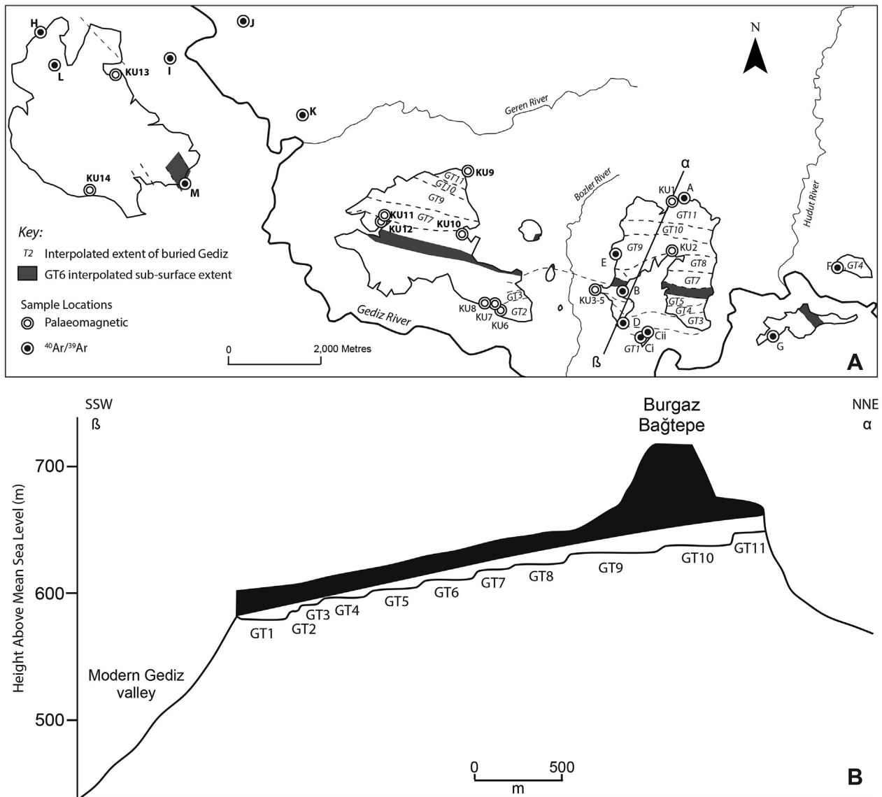
Fig. 4. A. Map of the buried Early Pleistocene terraces GT11–GT1 based upon Maddy et al. (2012a). Also shown are the sampling locations for the ^{40}\text{Ar}/^{39}\text{Ar} age estimates (A–M) and the palaeomagnetic sampling KU1–KU14. New samples reported here for the first time are shown in bold. A simplified section ( \alpha – \beta ) showing the stepped Ahmetler–Gediz gravel contact (GT terrace bases) on the Burgaz plateau is shown in B below.
