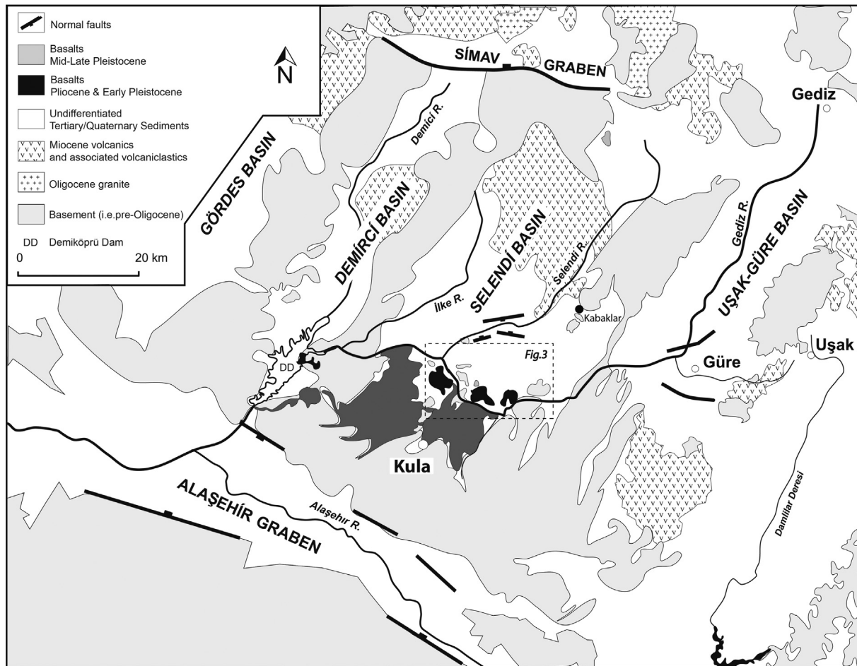
Fig. 2. Simplified geology of the Gediz River Basin showing the location of the Neogene Basins and their relationship to the basement rocks of the Mendere Massif. Basalts show the approximate extent of the Kula Volcanic Province. Dashed box shows the approximate position of Fig. 3.
