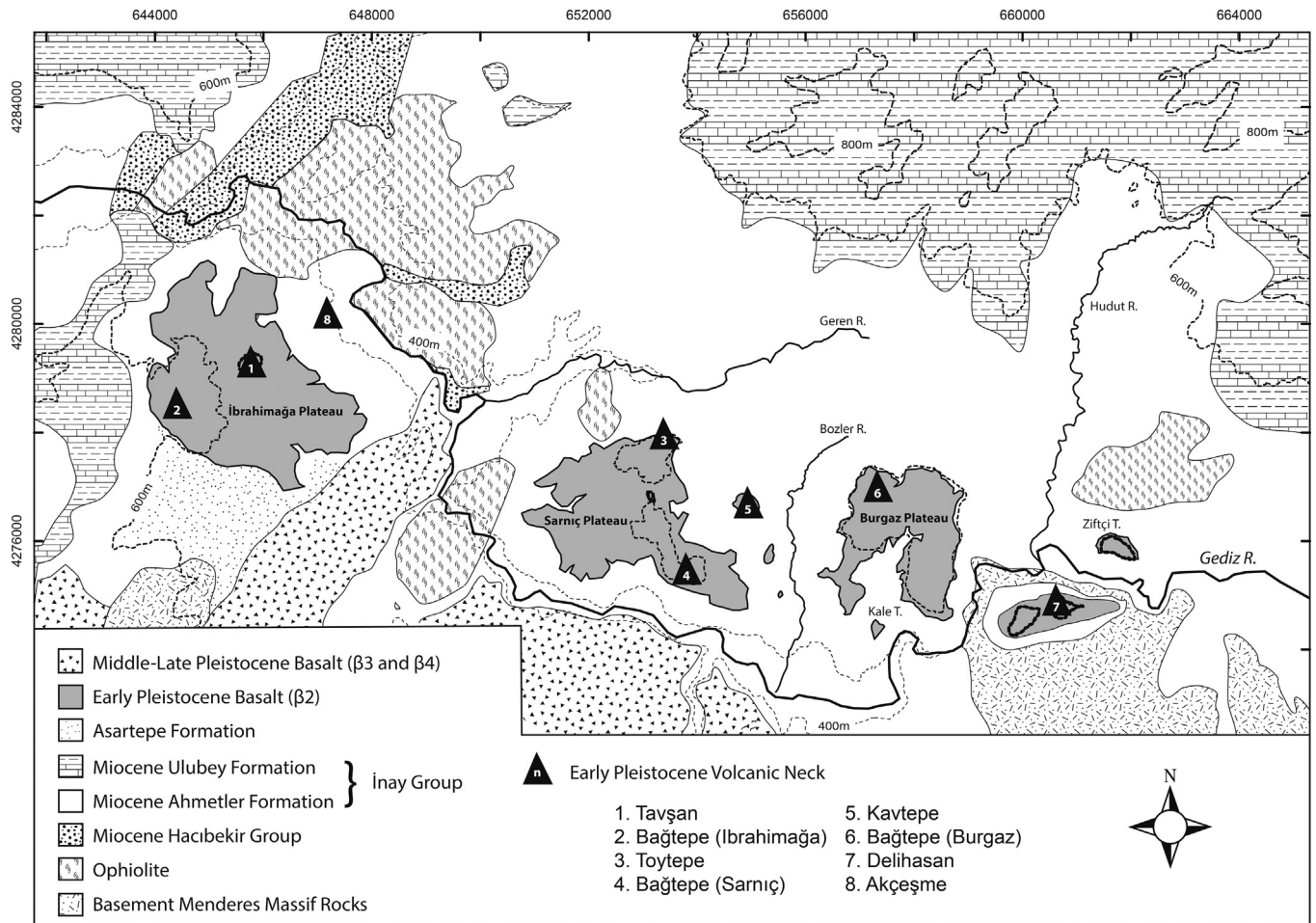
Fig. 3. Generalized geology of the study area (based on Ercan et al., 1983 with modifications). Coordinates are UTM Zone 35.
