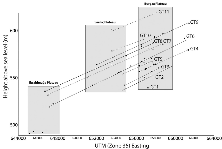
Fig. 6. Terrace base longitudinal profiles for terraces of the Gediz Valley Formation (Maddy et al., 2012a). Sample points represent accurately surveyed height marking the contact between Gediz River gravels of the terraces and the underlying Ahmetler Fm. Shaded boxes signify the approximate extent of the high level basaltic plateaux.
