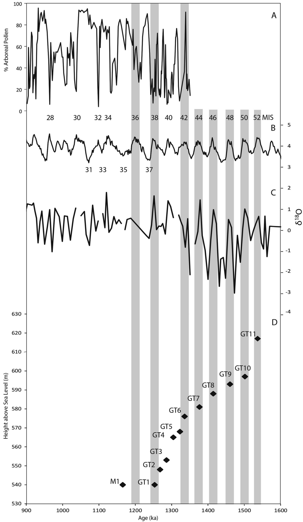
Fig. 10. Proposed correlation of: A) the regional pollen record from Tenaghi Philippon (Tzedakis et al., 2006), B) the \delta^{18}O stacked record of Lisiecki and Raymo (2005); C) the regional \delta^{18}O record from ODP967 (Kroon et al., 1998) and D) the terrace base altitudes and chronology derived from Table 4.
