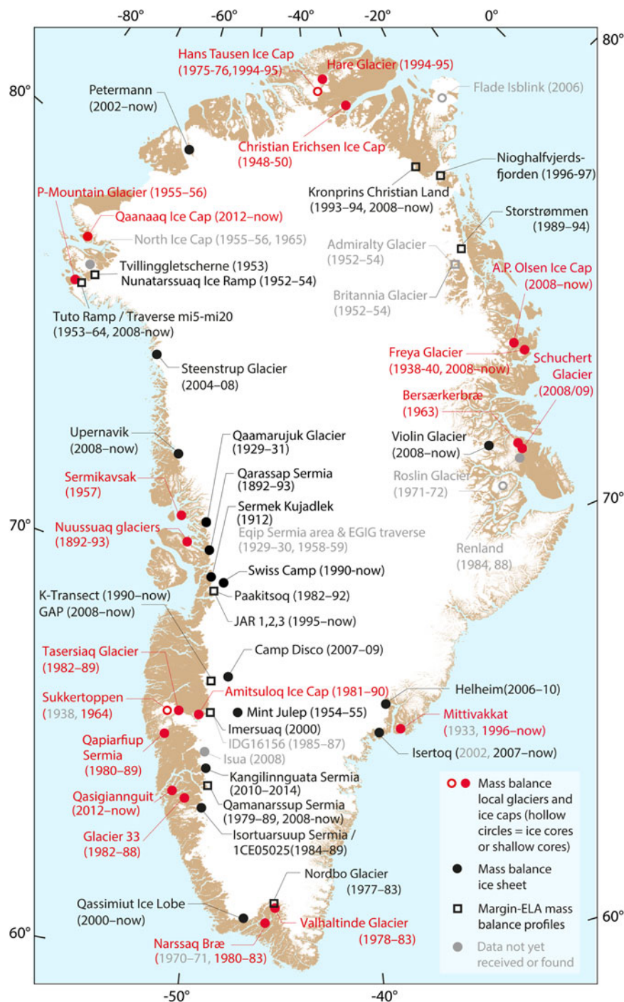
Fig. 1. Map of Greenland showing location and duration of observation of all currently known surface mass-balance sites located in the ablation area of the ice sheet and on the local glaciers (a considerable number of the entries are on the basis of Weidick, 1995).
