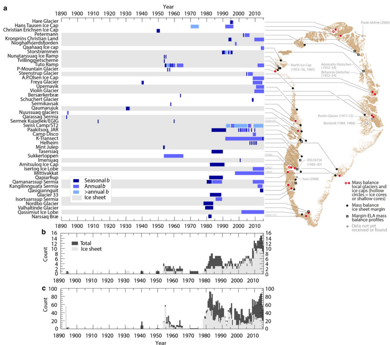
Fig. 4. Overview of the data currently contained in the surface mass-balance database. (a) Temporal availability of data for each site and temporal resolution of the data. (b) Number of active measuring sites over time. (c) Number of active measuring points over time.
