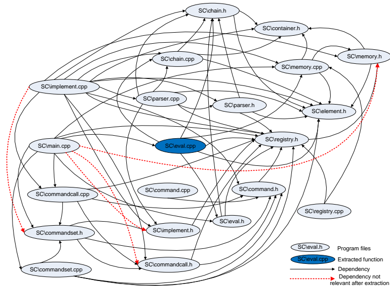
Figure 4.5: Dependency Graph
