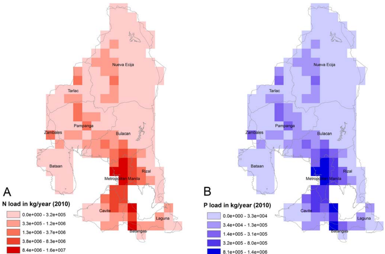
Fig. 4. (A) Nitrogen load and (B) phosphorus load map for the year 2010 (baseline scenario) for the whole Manila Bay watershed in kg N or P per year
