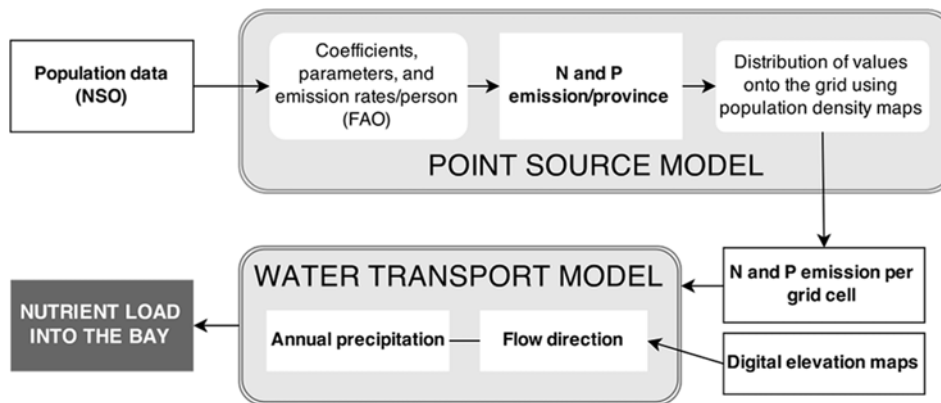
Fig. 2. Point source and nutrient load model flow chart
