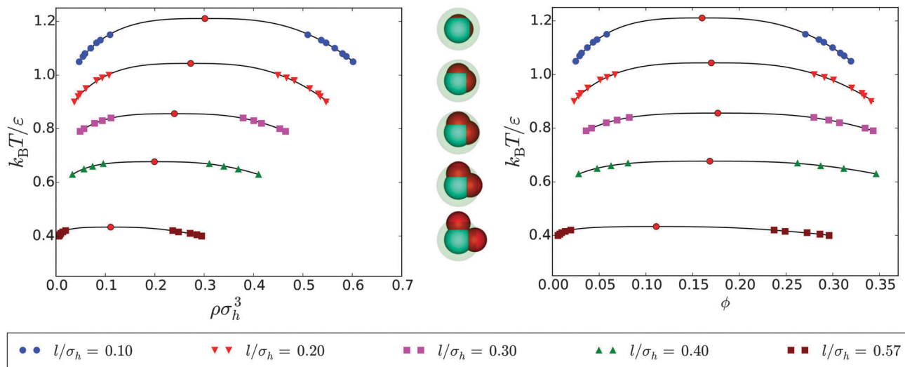
Fig. 2 Gas-liquid coexistence curves for MMSW particles. We provide both the temperature k_B T/\epsilon – density \rho\sigma_h^3 , and temperature k_B T/\epsilon – packing fraction \phi representation. The packing fraction is calculated as \phi = Nv_p/V , with v_p the particle volume as discussed in Appendix. The labels stand for different increasing values of the bond length l . The full red dots indicate the location of the critical points by eqn (7).
