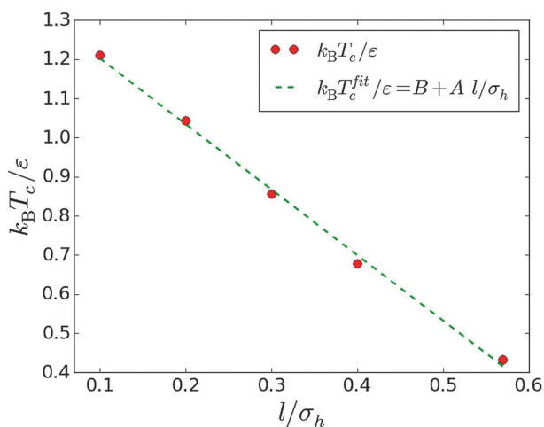
Fig. 3 Critical temperature k_B T_c/\epsilon (full red dots) as a function of bond length l/\sigma_h . The green dashed line shows the linear fit to the data for the critical temperature k_B T_c^{\text{fit}}/\epsilon = B + A l/\sigma_h , with B = 1.37 and A = -1.67 , indicating a linear relation between the bond length “knob” and the system’s critical temperature.
